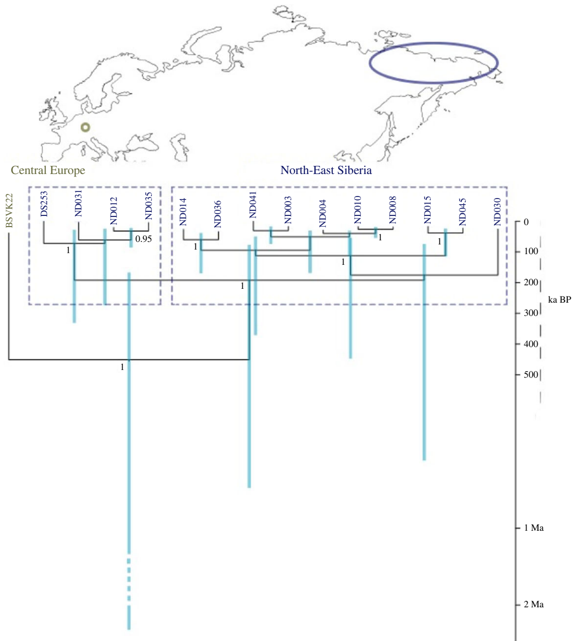
Figure 1. Bayesian phylogeny of the sequence from Bockstein-Loch (BSVK22) in relation to previously published sequences of woolly rhinoceroses ( Coeledonta antiqutatis ) from Eastern Siberia [11]. Support values greater than 0.95 are shown.
