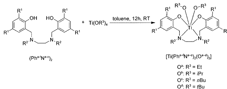
Scheme 2. Synthesis of titanium salan complexes by metalation with different titanium alkoxides. [43,46,47]
