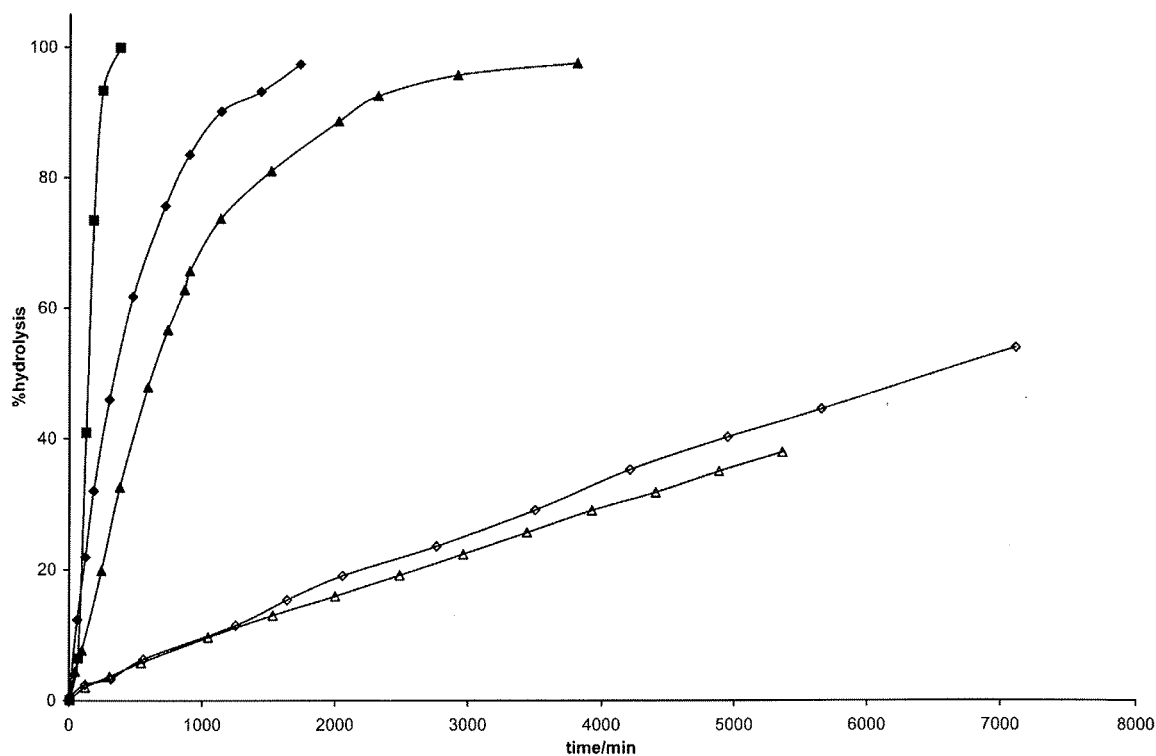
Figure 8. Plots of hydrolysis vs. reaction time for [\text{Ti}(\text{Ph}^{\text{tBuN}^{\text{Me}}})_2(\text{O}^{\text{iPr}})_2] (■), [\text{Ti}(\text{Ph}^{\text{F}^{\text{N}^{\text{Me}}})}_2(\text{O}^{\text{iPr}})_2] (◆), [\text{Ti}(\text{Ph}^{\text{MeN}^{\text{Me}}})_2(\text{O}^{\text{iPr}})_2] (▲), [\text{Ti}(\text{Ph}^{\text{ClN}^{\text{Me}}})_2(\text{O}^{\text{iPr}})_2] (◇), [\text{Ti}(\text{Ph}^{\text{BrN}^{\text{Me}}})_2(\text{O}^{\text{iPr}})_2] (△). Data acquired by time-resolved ^1\text{H} NMR spectroscopy at 37^\circ\text{C} . Data gathered by monitoring the decrease in isolated signals of the titanium-bound salan backbone and the increase in the signals from the liberated alkoxy ligands. Integrals are normalized against the internal standard.
