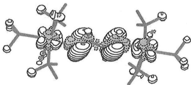
Fig. 6 Computed electron density differences for the first oxidation of the model complex [\{\text{RuCl}(\text{CO})(\text{PH}_3)_3\}_2(\mu\text{-CH}=\text{CH}-\text{CH}=\text{CH})] ( 2^{\text{H}} ); loss of electron density is shown in white and an increase is shown in grey
