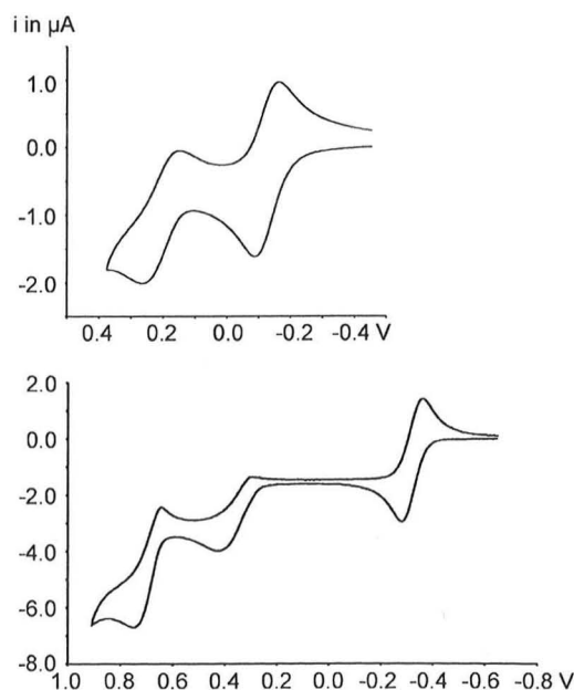
Fig. 1 Voltammetric traces for complexes 1 ( v=0.2 \text{V s}^{-1} , 293 K, upper trace) and 2 ( v=0.1 \text{V s}^{-1} , 195 K, lower trace) in \text{CH}_2\text{Cl}_2/\text{NBu}_4\text{PF}_6 .
