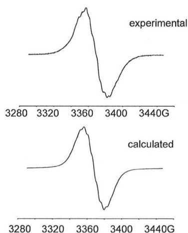
Fig. 5 Experimental and calculated ESR spectrum of electrogenerated I + in fluid solution (CH 2 Cl 2 , 303 K)
