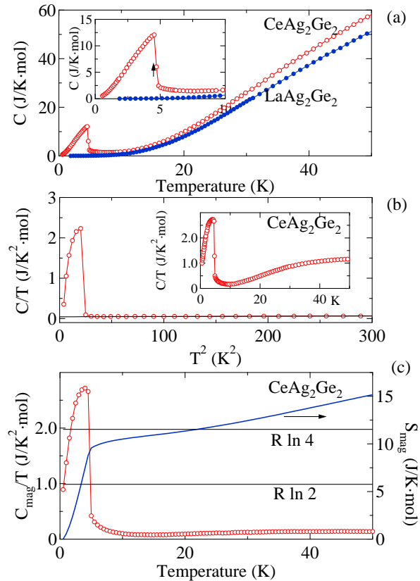
FIG. 6: (Color online)(a) Temperature dependence of the specific heat of \text{CeAg}_2\text{Ge}_2 and \text{LaAg}_2\text{Ge}_2 , the inset shows the low temperature part, (b) specific heat of \text{CeAg}_2\text{Ge}_2 in the form of C/T vs. T^2 after subtracting the schottky and the 4f contribution, the solid line shows the extrapolation of the high temperature specific heat to 0 \text{ K} , inset shows C/T versus T and (c) magnetic specific heat C_{\text{mag}} in the form of C_{\text{mag}}/T vs. T together with the magnetic entropy S_{\text{mag}} .
