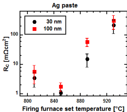
Figure 4: Specific contact resistance for Ag paste in dependence on the firing furnace set peak temperature for 30 and 100 nm thick doping layers
