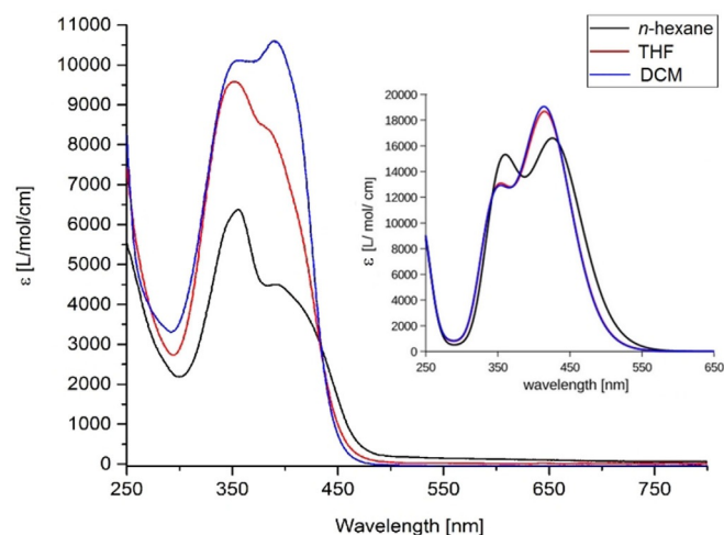
Figure 4. Experimental absorption spectra of 6 . Inset: Calculated absorption spectra of 6 using empirically corrected CAM-B3LYP/cc-pVDZ TD-DFT excitation energies at PBE0/def2-TZVP structures and a Gaussian broadening of FWHM = 0.25 eV.
