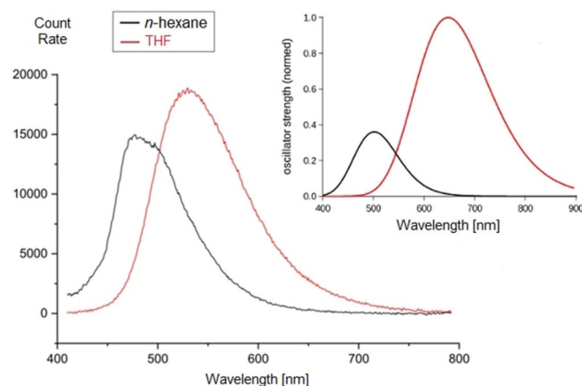
Figure 5. Experimental fluorescence spectra of compound 6 . Inset: Calculated emission spectra of 6 at wB97XD/def2-TZVP TD-DFT level of theory. Oscillator strengths were normalized to 1.0 at \lambda_{\text{max}} in THF.
