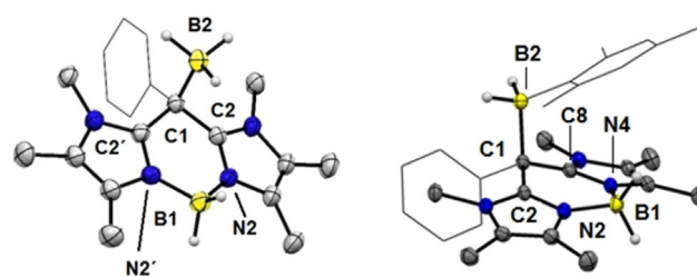
Figure 6. Molecular structure of compounds 12 (left) and 14 (right). The phenyl and mesityl entity are represented in the wireframe model. Thermal ellipsoids are drawn at the 50% probability level. Carbon bound hydrogen atoms are omitted. The illustrated molecule for 12 is located on a crystallographic mirror plane containing B1, C1, B2 and the phenyl entity. Selected bond lengths [Å] and bond angles [°] for 12 : B1–N2 1.5443(16), C1–C2 1.4975(14), C2–N2 1.3330(15), C1–B2 1.679(2), C2–C1–C2' 108.16(13), C2–C1–B2 106.34(9), N2–B1–N2' 105.03(14); for 14 : B1–N2 1.5519(17), B1–N4 1.5543(18), C1–B2 1.734(2), C2–N2 1.3368(16), C8–N4 1.3340(16), C1–C2 1.5033(18), C1–C8 1.4989(17), N2–B1–N4 104.24(10), C8–C1–C2 107.40(10).
