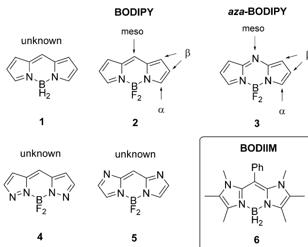
Scheme 1. Structures of compounds 1–6.
