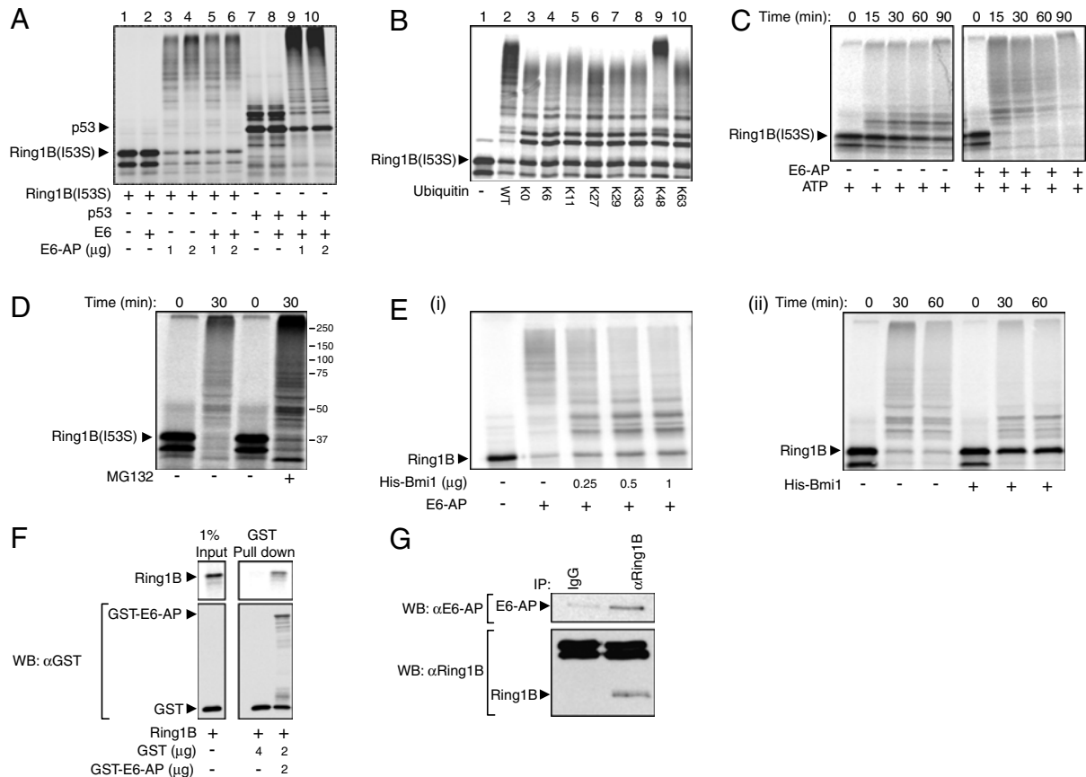
Fig. 2. Ring1B is ubiquitinated and targeted for degradation by E6 AP in vitro. (A) In vitro translated and ^{35}\text{S} labeled Ring1B I53S and p53 were ubiquitinated in a cell free reconstituted system in the presence or absence of recombinant E6 and His E6 AP as indicated. (B) ^{35}\text{S} labeled Ring1B I53S was conjugated in a cell free reconstituted system in the presence of ubiquitin species that contain the indicated lysine residues. (C and D) ^{35}\text{S} labeled Ring1B I53S was subjected to in vitro degradation in the presence of ATP and an ATP regenerating system, E6 AP, and MG132 (20 μM) as indicated. (E) Ubiquitination and subsequent degradation of Ring1B by E6 AP is inhibited by the addition of Bmi1. ^{35}\text{S} labeled Ring1B was subjected to in vitro ubiquitination (i) and degradation (ii) in the presence of His E6 AP and His Bmi1 as indicated. Conjugation and degradation assays were carried out as described under Materials and Methods . The SDS PAGE resolved proteins were visualized via PhosphorImaging. (F) ^{35}\text{S} labeled WT Ring1B was pulled down by GST or GST E6 AP using glutathione beads. The SDS PAGE resolved proteins were visualized using PhosphorImaging (Ring1B) or following Western blotting (GST). (G) Endogenous Ring1B was immunoprecipitated from U2OS cell extract using a specific antibody. The precipitates were resolved via SDS PAGE and analyzed for the presence of E6 AP and Ring1B using specific antibodies.
