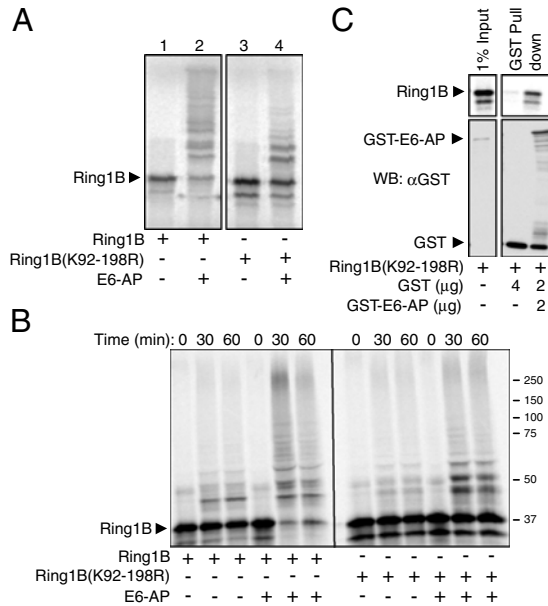
Fig. 3. The lysine residues in Ring1B that are self ubiquitinated and are essential for its histone H2A ligase activity are also ubiquitinated by E6 AP. (A and B) In vitro translated and ^{35} S labeled WT Ring1B or Ring1B (K92 198R) were subjected to ubiquitination (A) or degradation (B) in a cell free reconstituted system in the presence of recombinant His E6 AP as described under Materials and Methods . (C) ^{35} S labeled Ring1B(K92 198R) was pulled down by GST or GST E6 AP as described in the legend to Fig. 2F.
