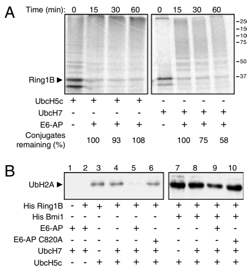
Fig. 4. The activating self ubiquitination of Ring1B protects it from targeting by E6 AP, and E6 AP ubiquitination of Ring1B inhibits its activity as histone H2A ligase. (A) In vitro translated and ^{35} S labeled Ring1B was preincubated with UbcH5C (can promote both self and E6 AP mediated ubiquitination) or UbcH7 (can promote only E6 AP mediated ubiquitination) in a cell free reconstituted system. Recombinant His E6 AP and reticulocyte lysate (as a source of proteasomes) were then added for the indicated times. The SDS PAGE resolved proteins were visualized via Phosphorimaging. (B) Nucleosomes were subjected to ubiquitination in a cell free reconstituted system in the presence of the indicated bacterially purified proteins as described under Materials and Methods . Monoubiquitinated histone H2A was detected using a specific antiubiquitinated histone H2A antibody.
