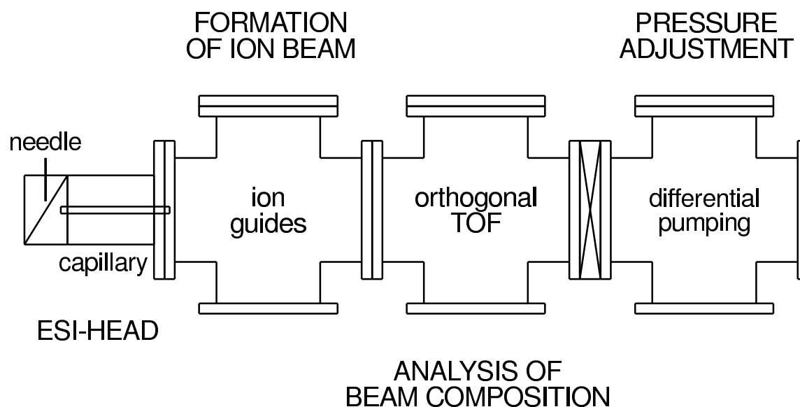
Figure 4.1: Schematic side view of the ESI deposition source for the soft-landing of sensitive analyte ions under UHV conditions.
