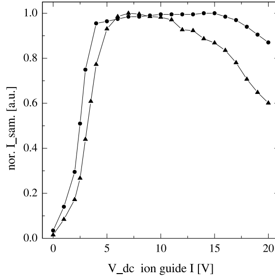
Figure 4.19: Normalized analyte current I_{sam.} versus the dc component V_{dc} IG I of the applied rf signal. The rhodamine 6G I-V curve is marked by ▲, whereas the bovine albumin I-V curve is denoted by ●. The value of V_{skim.} was set to +25 V during the experiment.
