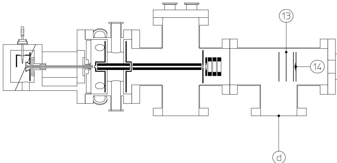
Figure 5.1: Deposition geometry during sample preparation: A special deposition chamber (d) with a funnel lens system (13) in front of the substrate (14) are used to guide and to deposit the analyte ions onto the substrate.
