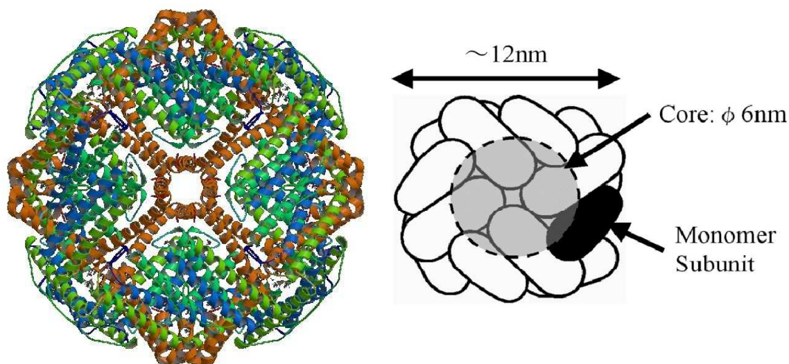
Figure 5.14: Ribbon diagram and structural schematic of horse spleen ferritin. Schematic drawing reproduced from [54].
