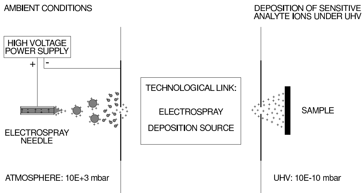
Figure 1.1: Schematic drawing of the ESI-deposition circuit: After the generation of a charged aerosol and successive ESI in atmospheric conditions, the electro spray deposition source acts as vacuum technological link between atmosphere and UHV, where the deposition of the charged analyte ions takes place.
