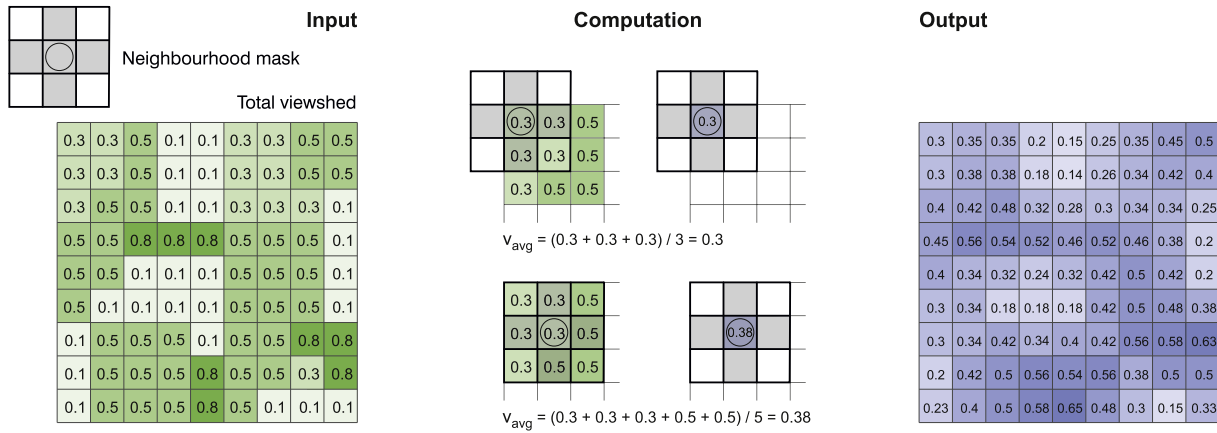
Fig. 4. Example of the VNC analysis process: a neighbourhood mask representing the VNC theory and a total viewshed are taken as input, in the computation phase the mask focuses on each cell of the total viewshed and writes the result of the evaluation method (in this case average visibility) to a new output raster file.
