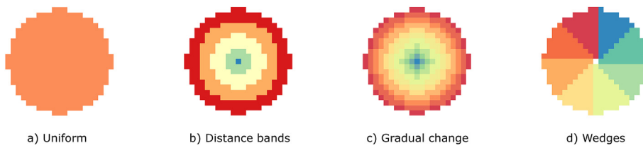
Fig. 1. Example representations of VNCs with different structures where groups of cells are indicated by different colours: an assumption about the visual property values is formulated for each group of cells. (For interpretation of the references to colour in this figure legend, the reader is referred to the Web version of this article.)
