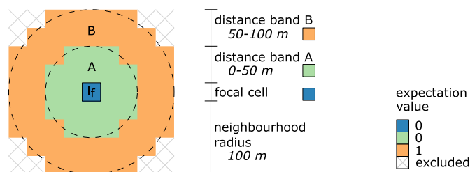
Fig. 2. VNC of an example hypothesis where archaeological features are located in invisible places surrounded by highly visible locations. This can be expressed by considering a low expectation value for distance band A and a high one for band B.
