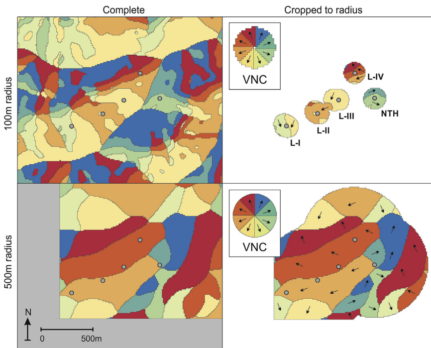
Fig. 9. The rows show results of the two experiments performed in Analysis 1. The left column shows the results for all cells. The right column shows the same results but only for those cells within a 100 m (top row) or 500 m radius (bottom row). The colours and arrows indicate per cell the direction in which the wedge with the highest average visibility is located. Notice how the top row shows the sites are located in the direction with highest visibility within 100 m, whereas the bottom row shows the sites are not located in the direction with highest visibility within 500 m. (For interpretation of the references to colour in this figure legend, the reader is referred to the Web version of this article.)
