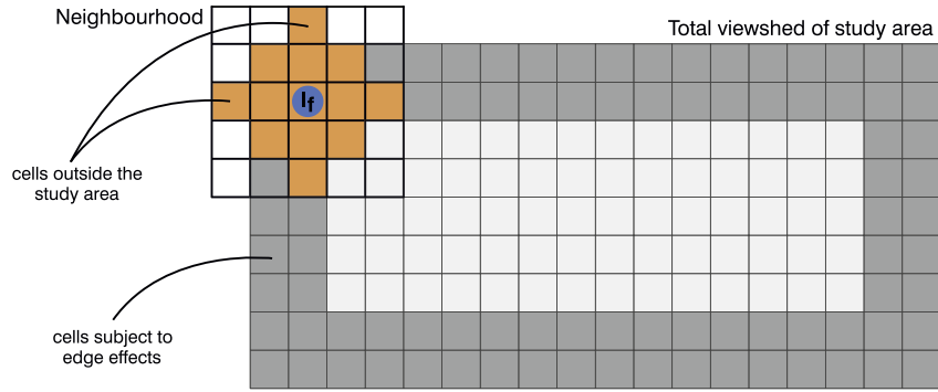
Fig. 3. Example of a cell whose neighbourhood extends beyond the input total viewshed defining the study area. When interpreting VNC analysis results, such cells should be excluded to remove edge-effects.
