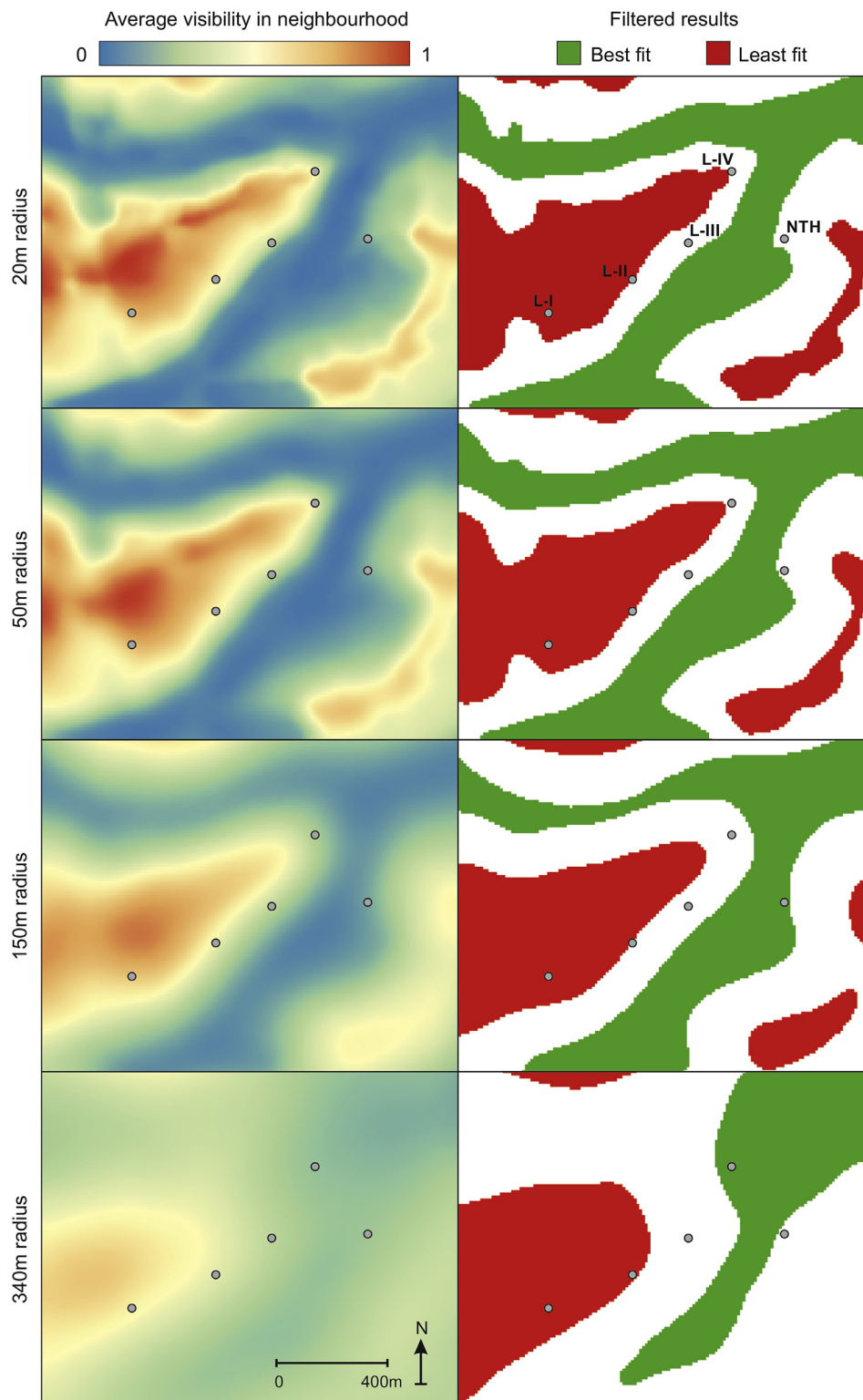
Fig. 7. The rows show results of the four experiments performed in Analysis 1. The left column shows the precise results per cell ranging between 0 and 1 (i.e. low to high average visibility in neighbourhood). The right column shows the same results grouped in the lower quartile in green (locations offering the best fit with the hypothesis of low average visibility) and the upper quartile in red (worst fit). (For interpretation of the references to colour in this figure legend, the reader is referred to the Web version of this article.)
