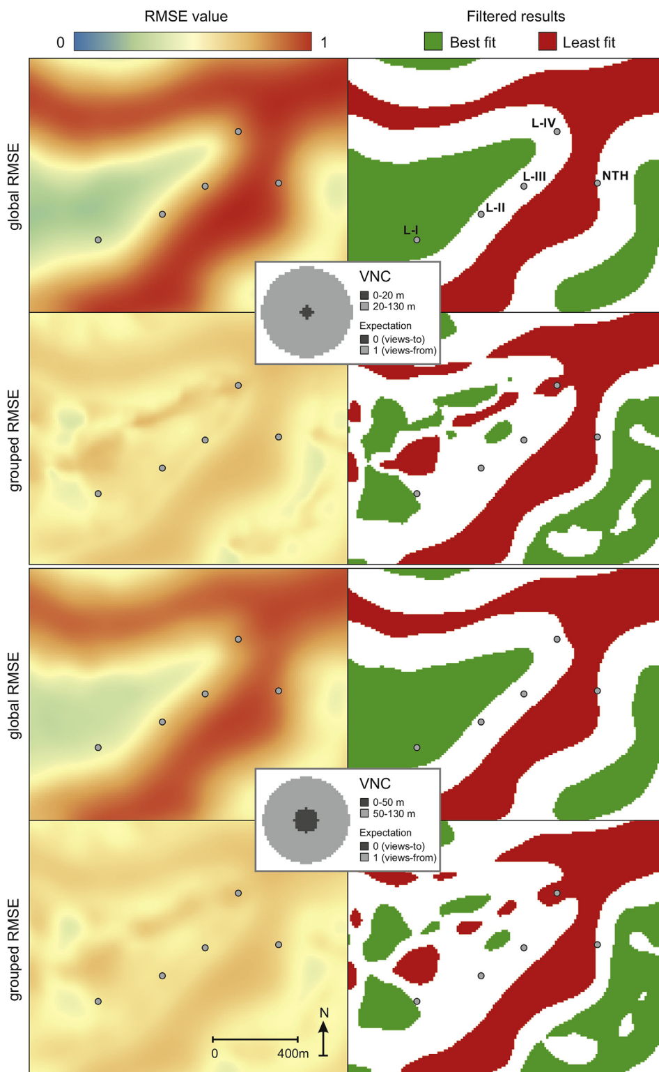
Fig. 8. The rows show results of the four experiments performed in Analysis 2. The top two rows use a VNC with an inner radius of 20 m, and the bottom two rows use an inner radius of 50 m. The left column shows the precise results per cell ranging between 0 and 1 (i.e. low to high RMSE value). The right column shows the same results grouped in the lower quartile in green (best fit between expectation and total viewshed) and the upper quartile in red (worst fit). (For interpretation of the references to colour in this figure legend, the reader is referred to the Web version of this article.)
