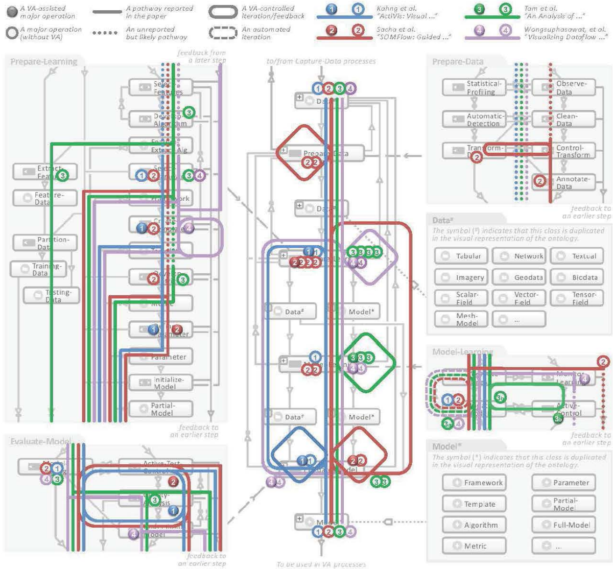
Fig. 6. Pathways within our ontology illustrated for the examples 1-4 of Table 1. The pathways are complemented with marked “bus stops” illustrating exactly at which stages visualization is used to improve the ML workflow.
