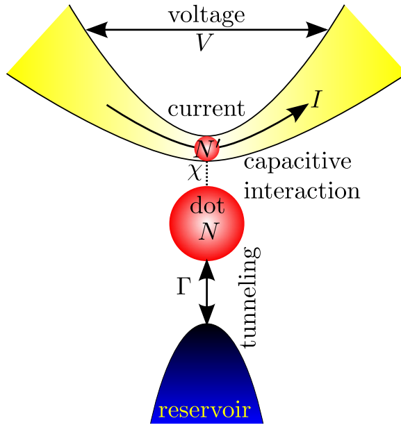
Figure B.1. The model of detecting the dot's charge. An electric junction contains another dot with effective occupation N' , coupled capacitively to the measured dot. The fluctuations of the current I in the junction biased by the voltage V depend on the dot's occupation N with the proportionality constant \chi .
