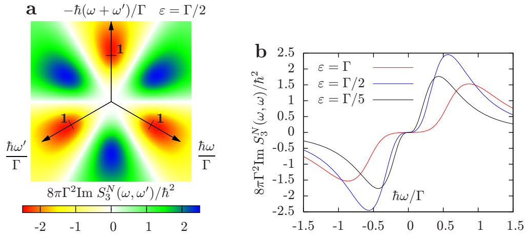
Figure 4. Time asymmetry of the third-order correlation of dot occupation fluctuations S_3^N(\omega, \omega') in frequency domain at kT \ll \Gamma . The symmetry is broken if \text{Im}S_3^N \neq 0 . (a) For \varepsilon/\Gamma = 0.5 and arbitrary \omega, \omega' the asymmetry vanishes (white lines) when \omega, \omega' or \omega + \omega' is equal to 0. The hexagonal structure reflects the symmetry under permutations of frequencies. (b) Taking different values \varepsilon/\Gamma = 1, 0.5, 0.2 and \omega = \omega' it is clear that the maximal asymmetry occurs for energy/frequency parameters of the same order.
