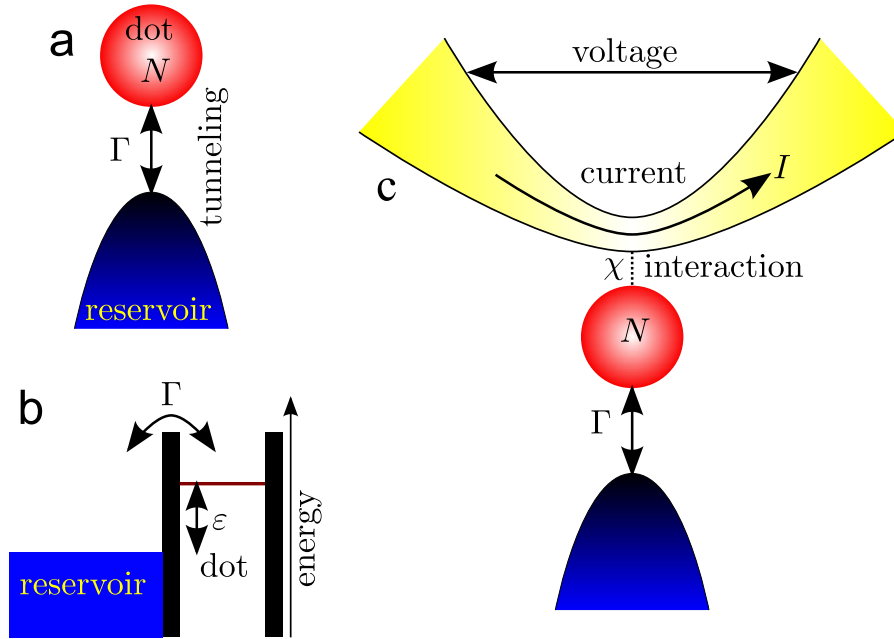
Figure 3. (a) The system consists of the dot (red) exchanging the elementary charge with a reservoir (blue). (b) The diagram of energy levels. At zero temperature, the Fermi sea of blue levels is full but electrons may still jump on and off the dot's red level. (c) Proposed detection by an electric junction (yellow). The junction and dot are weakly coupled capacitively and the directly measured quantity is the current I through the junction biased with the voltage. The charge is allowed to jump between the dot and the lower reservoir but not the junction.
