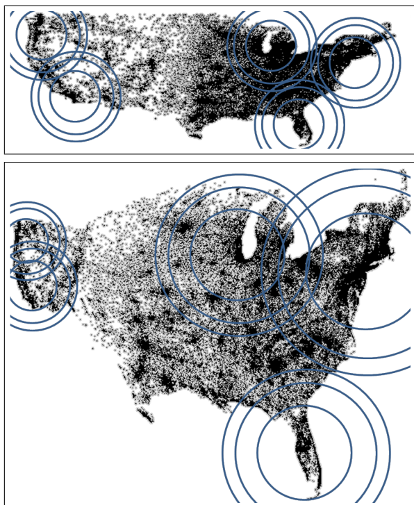
Fig. 1. RadialScale distortion technique applied to the USA census data. Only a few circles are displayed to show the schematic idea of the algorithm. (a) Original USA census data with regular circular bins. (b) Distorted map with adjusted circular bins and data point location.
