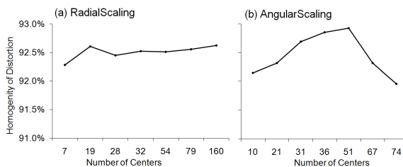
Fig. 6. Homogeneity measure for the RadialScale (a) and AngularScale (b) technique using multiple center points.
