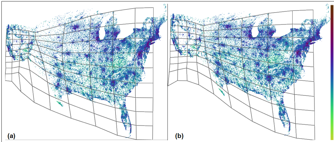
Fig. 3. RadialScale using (a) 19 center points and (b) 28 center points based on local maxima for the distortion.
