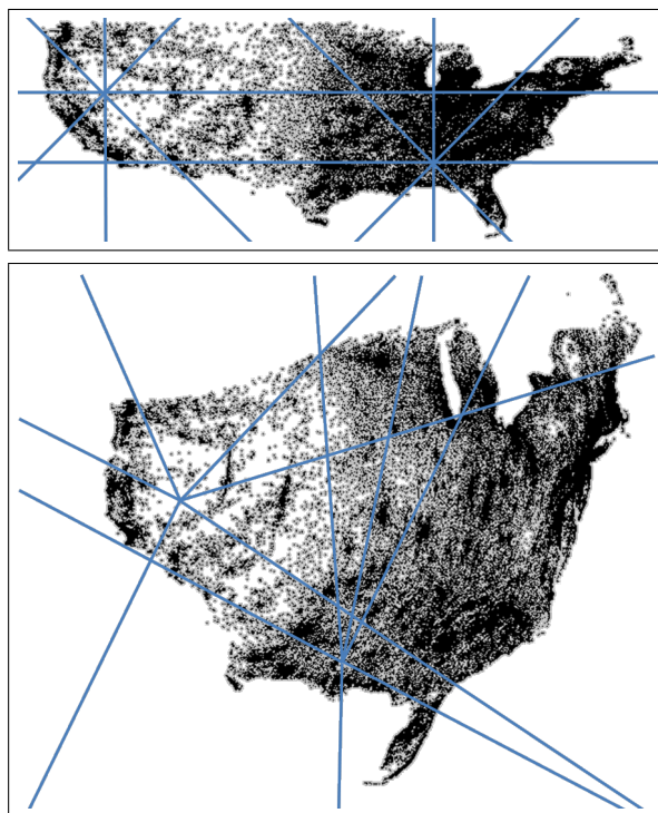
Fig. 2. AngularScale distortion technique applied to the USA census data based on local minima. The angular-lines only aim at showing the schematic idea of the algorithm. (a) Original USA census data with regular angular segments. (b) Distorted USA census data with adjusted angular segments and data point location.
