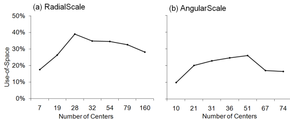
Fig. 5. Use-of-Space for the RadialScale (a) and AngularScale (b). The measure is best when it is high which means a better use of the screen space.
