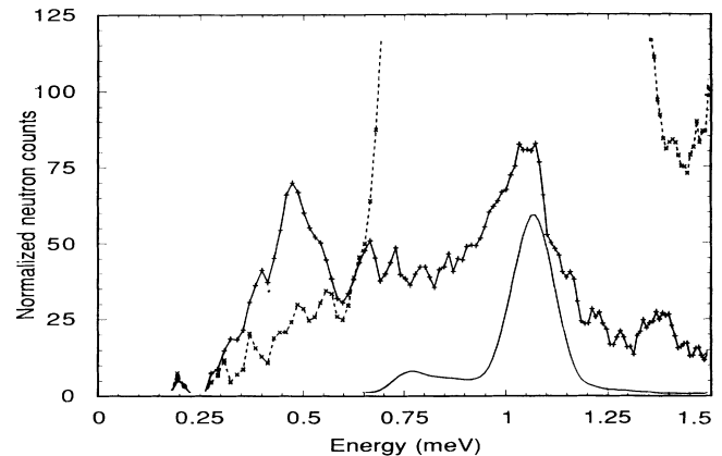
FIG. 2. Inelastic spectrum (arbitrary units) for Q = 0.8 \text{ \AA}^{-1} as a function of energy. The solid line with '+'s corresponds to a coverage of 5.06 atomic layers. The ripplon peak is found at 0.47 \text{ meV} and the bulk phonon at 1.05 \text{ meV} . Dashed line with 'x's: spectrum with the cell filled with bulk liquid; note that the ripplon peak has disappeared. The full line shows the same spectrum divided by 100 (the feature at 0.75 \text{ meV} is due to multiple scattering).
