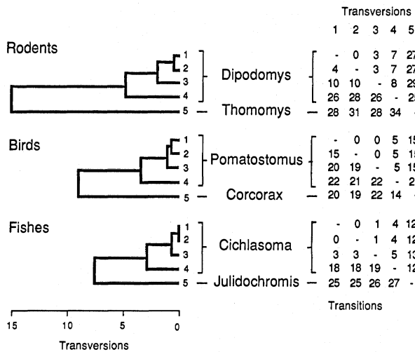
FIG. 3. Tree analysis of cytochrome b sequences in Fig. 2. Species labels correspond to Table 1. Numbers of transversion differences among pairs of species appear above the diagonal and numbers of transitions are below. The most parsimonious trees deduced by a character-state analysis of the data are shown. The branch lengths of the trees are drawn proportional to the number of transversions on each lineage, with each transition being considered equivalent to 0.1 transversion (24). These trees are consistent with previous concepts of phylogeny for these groups (25-27).
