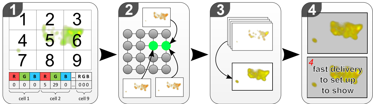
Fig. 2. Process pipeline to create self-organizing sentiment maps. The self-organizing sentiment map is determined by (1) extracting corresponding feature vectors, (2) calculating the best matching unit, (3) aggregating similar images according to the SOM, and finally (4) mapping the coherence and the additional information like the used terms to the images.
