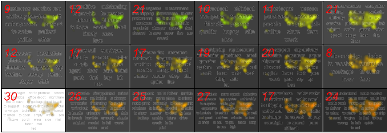
Fig. 1. Visualization of customer feedback data using sentiment analysis and self organizing maps. Term groups with different sentiment scores are visible and additionally the geospatial distribution of the terms is displayed. The brightness of the background represents the coherence of the geographic distribution for each SOM node.
