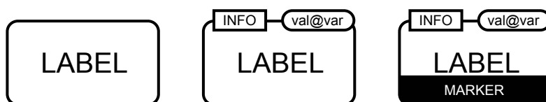
Figure 2.12: The Process Description glyph for macromolecule, shown plain and unadorned on the left, with an additional state variable and a unit of information in the middle, and with a labelled clone marker on the right.
