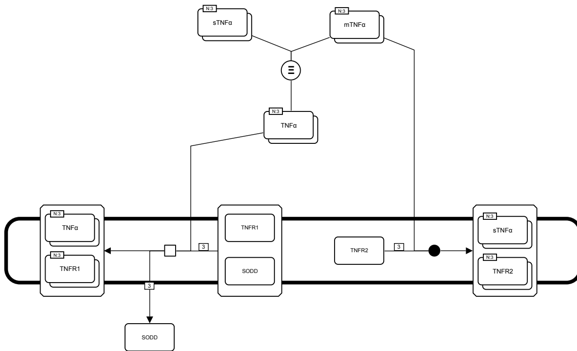
Figure 2.53: Binding of diverse forms of TNFα to TNF receptors.
