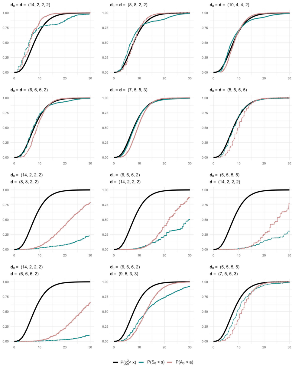
Figure 3. Null and non-null distributions of S_0 and A_0 , and the \chi_9^2 -distribution when some simple IEAS( \mathbf{d}_0 ) hypotheses are tested against IEAS( \mathbf{d} ) models for multigraphs with n = 4 and m = 10 .
