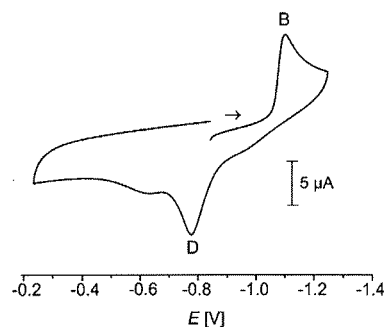
Figure 11. CV on the first reduction of 1 (peak B) and the associated return peak (peak D) in \text{CH}_2\text{Cl}_2/\text{CH}_3\text{CN} (3/1)/ \text{Bu}_4\text{NPF}_6^- solution at RT and \nu = 0.1 \text{ V s}^{-1} .
