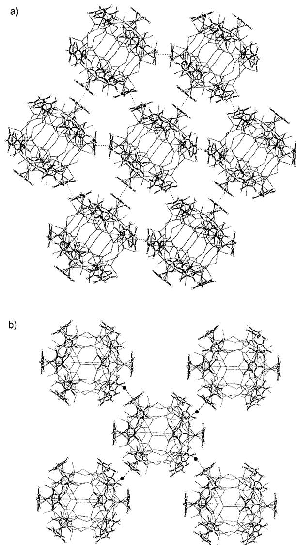
Figure 6. a) Fragment of a layer of [\text{Cp}^*\text{Fe}(\eta^5\text{-P}_3)]_{12}[\text{CuCl}]_{25}(\text{MeCN})_{10} molecules based on face-to-face and slipped \pi -stacking contacts \text{Cp}^*\cdots\text{Cp}^* of 3.54–4.42 Å in 4 , and b) on specific contacts \text{Br}\cdots\text{Cp}^* of \sigma - \pi type (3.36 Å) in 8 . Black balls denote bromine atoms participating in \sigma - \pi interactions; dashed lines show specific contacts. Hydrogen atoms and acetonitrile molecules are omitted; pseudo-spherical core atoms are shown by sticks.
