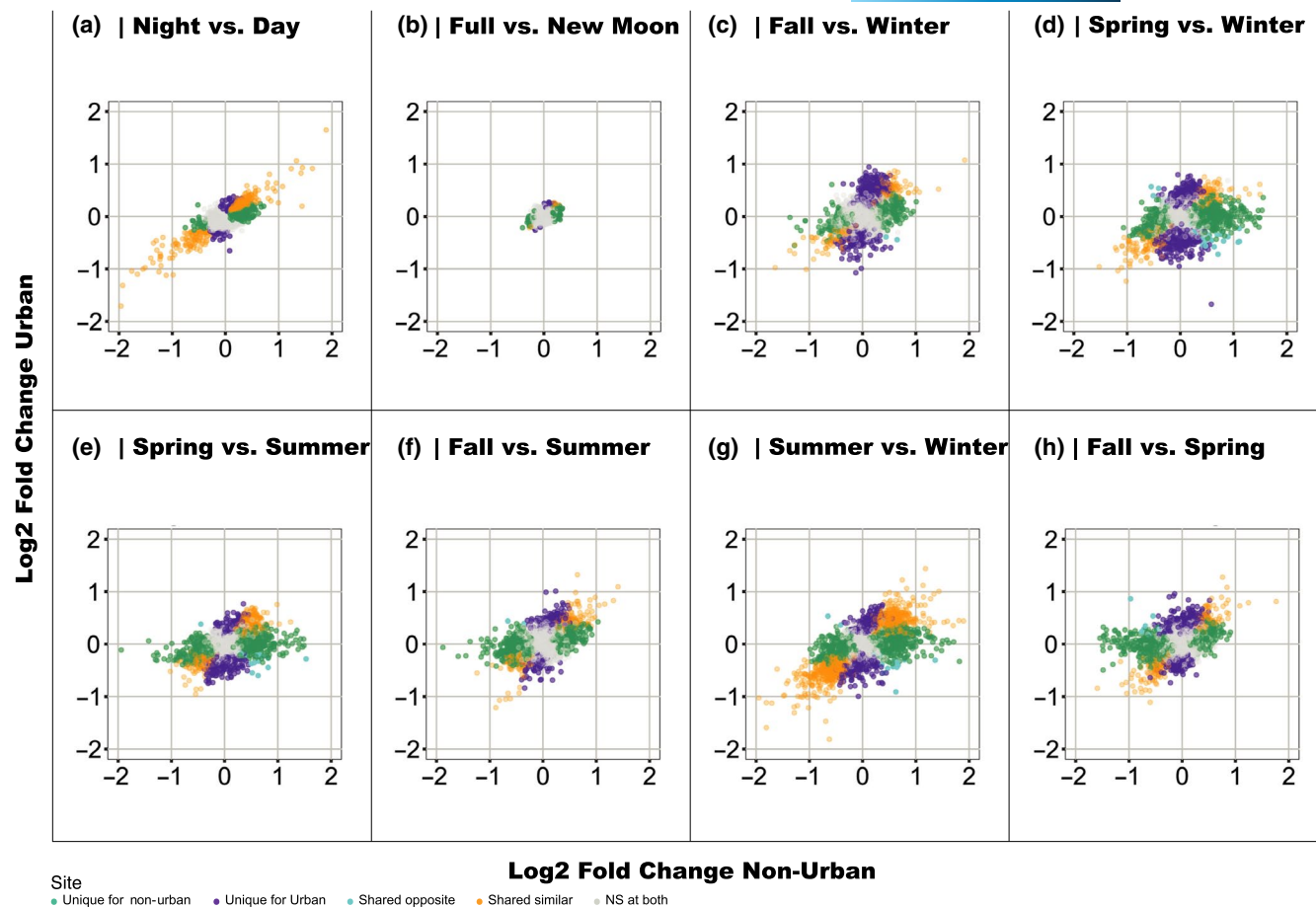
FIGURE 2 Scatter plot highlighting the transcriptomic response between non-urban and urban corals across diel, monthly, and seasonal cycles. The \log_2 fold change in the non-urban corals is represented on the x-axis. The y-axis shows the \log_2 fold change in the urban corals. Each gene is marked as a dot; unique differentially expressed genes of urban corals are highlighted in dark purple, unique differentially expressed genes for non-urban corals highlighted in dark green, and significantly differentially expressed genes in both areas: in light blue when expressed in the opposite manner, in yellow if expressed in the same manner in both areas and the non-significant gene were labeled as grey dots. Gene comparison is between the areas at the different cycles. (a) diel cycle, (b) monthly cycle and (c-h) seasonal cycle
