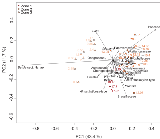
Figure 7. PCA biplot of terrestrial taxa from pollen analysis, showing a subset of 23 taxa, indeterminate and pre-Quaternary pollen, which explained most of the variance in the dataset. Sample depths (m) are coloured according to their corresponding zone. Explained variances of the two principal components (PC) are shown in brackets.
