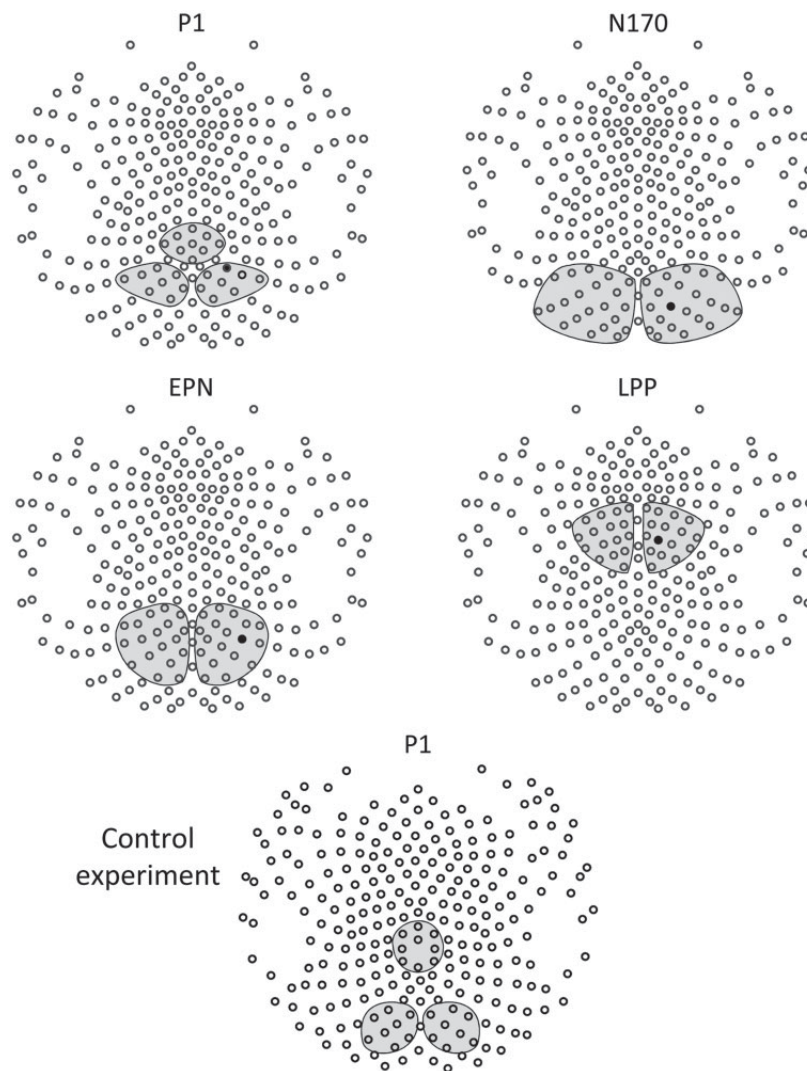
Fig. 4 Analyzed sensor clusters. Illustration of all sensor clusters as analyzed for each ERP effect. Black sensors indicate channels presented in detail in Figures 3 and 6. The sensor configuration is displayed from the top with the nose pointing up.
