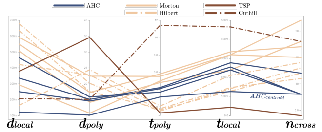
Figure 7: PCP plot showing the global ( d_{poly} & t_{poly} ), as well as local scores ( d_{local} , t_{local} & n_{cross} ), obtained using the interactions visible in Figure 4 (⑥ & ⑦) for different orderings for the NYC dataset.
