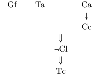
Figure 10.7: Graphical representation of the EOL formula \text{Gf} \wedge ((\text{Ta} \wedge (\text{Ca} \triangleleft \text{Cc})) \triangleleft \neg \text{Cl} \triangleleft \text{Tc}) .
