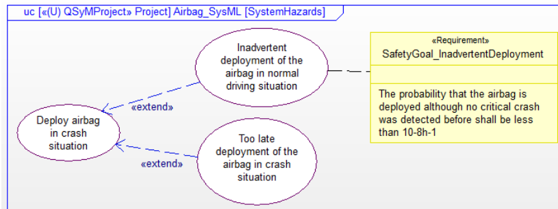
Figure 11.4: Safety goals generated in the Hazard Analysis and Risk Assessment.
