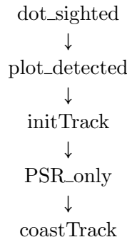
Figure 10.18: Graphical representation of the EOL formula \text{dot\_sighted} \wedge \text{plot\_detected} \wedge \text{initTrack} \wedge \text{PSR\_only} \wedge \text{coastTrack} .
