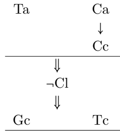
Figure 10.8: Graphical representation of the EOL formula (\text{Ta} \wedge (\text{Ca} \triangleleft \text{Cc})) \triangleleft \neg \text{Cl} \triangleleft (\text{Gc} \wedge \text{Tc}) .
