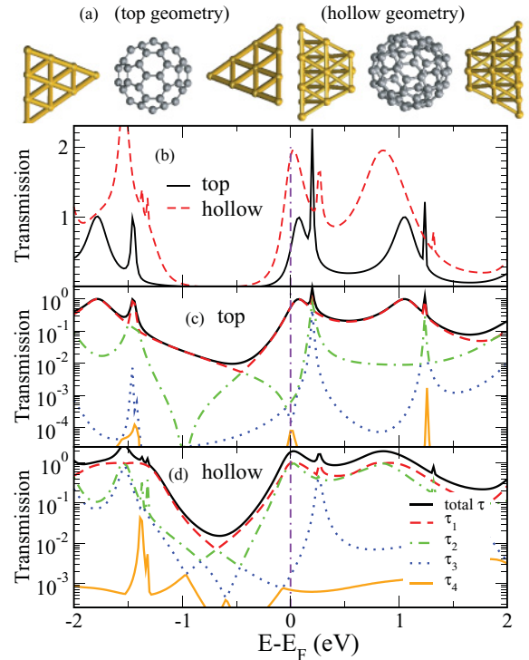
FIG. 1. (Color online) (a) Two ideal Au-C 60 -Au junctions with top (left) and hollow (right) binding geometries. (b) The transmission as a function of energy for the two geometries in (a). (c, d) The solid line corresponds to the total transmission, while the others correspond to the contribution of the individual transmission coefficients as a function of energy.
