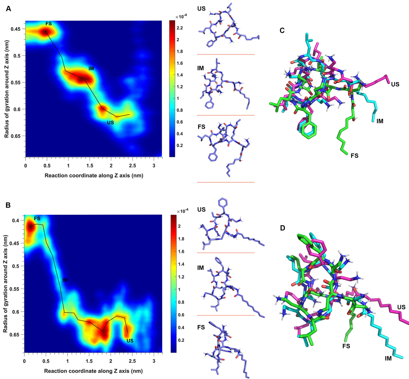
Figure 5. Conformational dynamics of octapeptin C4 (A) and FADDI-115 (B) in the outer membrane, with the superimposition of the octapeptin molecule at different conformational states shown for octapeptin C4 (C) and FADDI-115 (D). The conformational landscape is defined by sampling the radius of gyration of the octapeptin molecule around the z axis and the reaction coordinates of the penetration. The conformations of the octapeptin molecule are represented by points , and the color spectrum represents the density of points. The pathway of conformational transition from the unfolded state ( US ) to intermediate state ( IM ) and folded state ( FS ) is shown by a black line .
