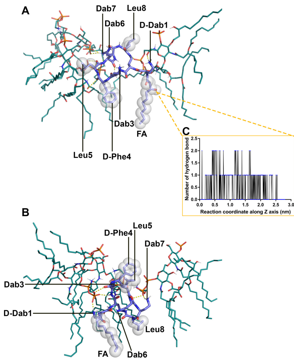
Figure 6. Interactions between the octapeptin and lipid A-pEtN molecules in the outer membrane. A , octapeptin C4. B , FADDI-115. C , the hydrogen bonds formed between the hydroxyl group on the fatty acyl chain of octapeptin C4 and the outer membrane lipids.
