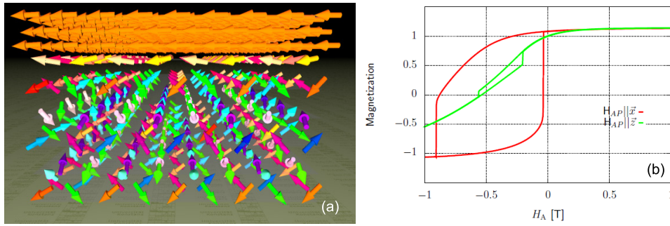
Figure 8. (a) Sketch of the magnetic state after in-plane field-cooling for a \text{Ru}_2\text{MnSi} ( L2_1 )/Fe interface. (b) In-plane and out-of-plane hysteresis loops of the \text{Ru}_2\text{MnSi} ( L2_1 )/Fe bilayers at 0 K [42].
