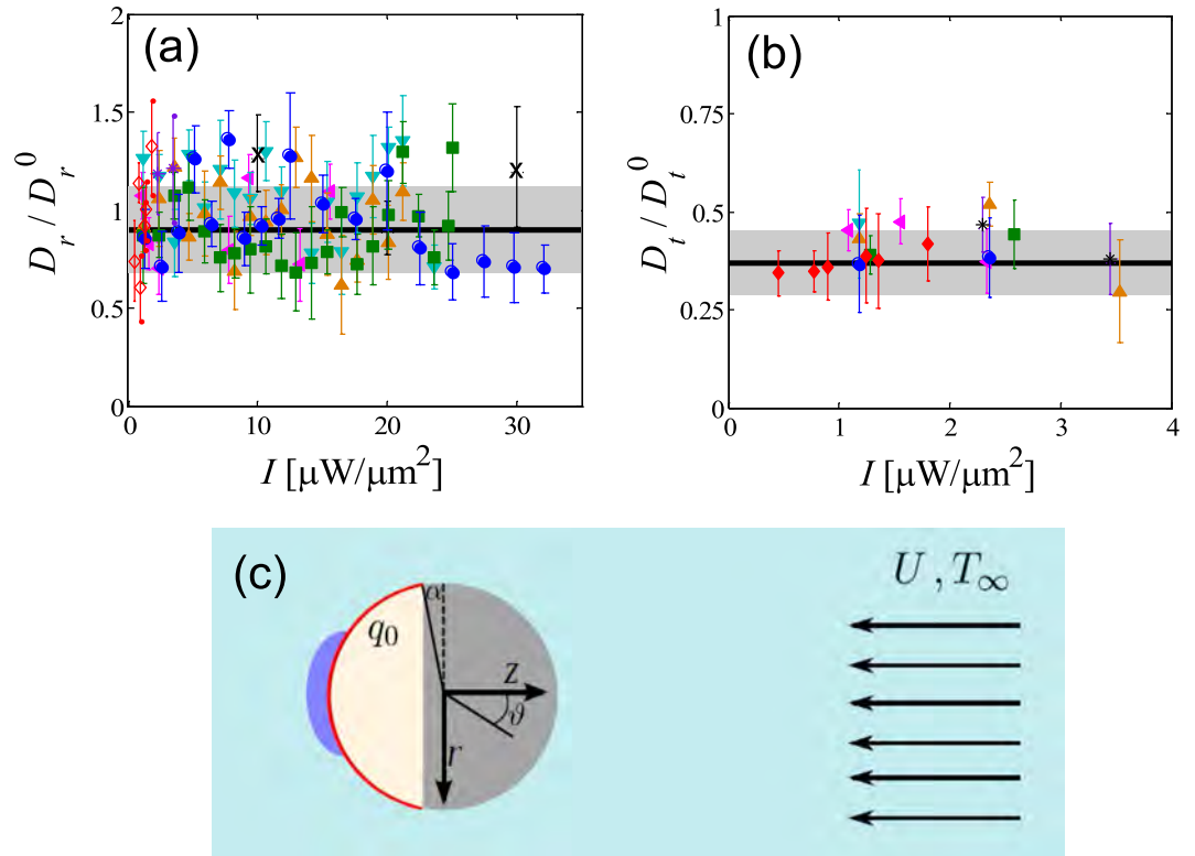
Figure 5. (a) Rotational and (b) translational diffusion coefficients of self-propelled colloids of different radii: R = 1.37 \mu\text{m} ( \triangleleft ), 1.63 \mu\text{m} ( \nabla ), 2.14 \mu\text{m} ( \triangle ), 2.45 \mu\text{m} ( \times ), 3.14 \mu\text{m} ( \square ), 3.88 \mu\text{m} ( ^\circ ), 8.02 \mu\text{m} ( * ), and 11.78 \mu\text{m} ( \diamond ), normalized by the corresponding Stokes-Einstein values in the bulk, and measured at different illumination intensities. The solid lines and the shaded areas represent the mean and the error, respectively, of D_r/D_r^0 and D_t/D_t^0 measured in absence of activity and averaged over all particles sizes. (c) Schematic illustration of a Janus particle immersed in a near-critical mixture with an ambient temperature T_\infty . Illumination of a thin carbon cap (red line) leads to a constant heat flux q_0 across the carbon cap. The ensuing demixing of a droplet near the cap propels the particle, such that the fluid velocity far from the particle is U in a frame-of-reference co-moving with the particle.
