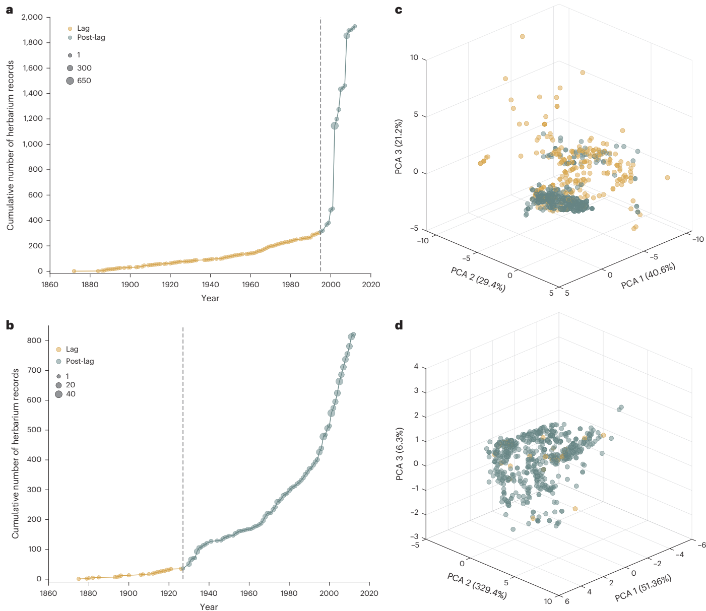
Fig. 2 | Biphasic temporal trends. a, b , Examples of biphasic temporal trends are represented by the invasions of Centaurea calcitrapa ( a ) and Chloris virgata ( b ) in Australia. c, d , While dissimilar climate conditions have been sampled during the lag and post-lag periods in C. calcitrapa ( c ), C. virgata exhibited analogous
