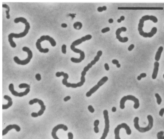
Fig. 3. Phase contrast photomicrographs of marine isolate strain GraTa2. Bar equals 10 \mu\text{m} for both prints
