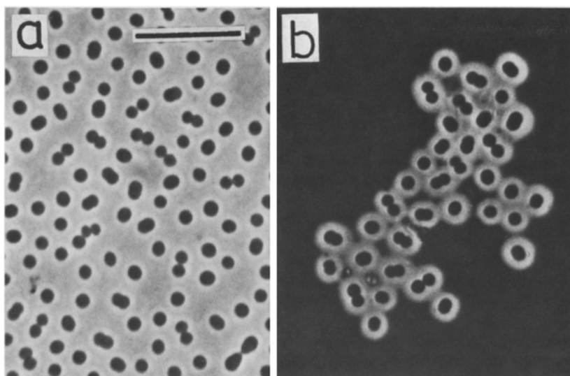
Fig. 1 Phase contrast photomicrograph of strain KoTa2. a Fresh culture grown on L-tartrate; b Indian ink preparation. Bar equals 10 \mu\text{m} for both prints
