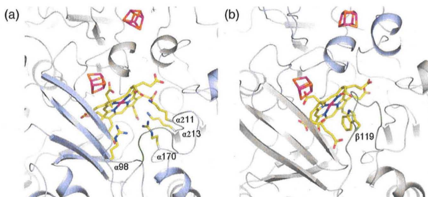
Fig. 5. Potential sulfite binding site. (a) At the functional siroheme-[4Fe-4S] center, the four key residues Arg \alpha 98 , Arg \alpha 170 , Lys \alpha 211 , and Lys \alpha 213 conserved in aSir and dSir constitute the pocket for binding sulfite and contribute significantly to catalysis. (b) At the structural siroheme-[4Fe-4S] center, the sulfite binding is blocked by a prolonged loop (in green) preceding strand \beta 126 : \beta 134 , from which the bulky side chain of Trp \beta 119 occupies the position of the substrate in front of the siroheme iron. For comparison, the equivalent loop in front of the functional siroheme-[4Fe-4S] center is also marked in green.
