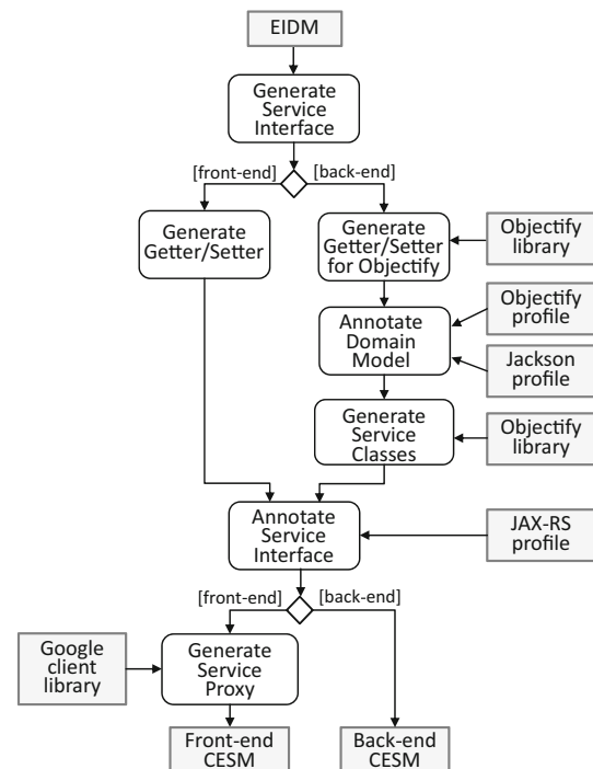
Fig. 19 Refinement of EIDM toward CESM
