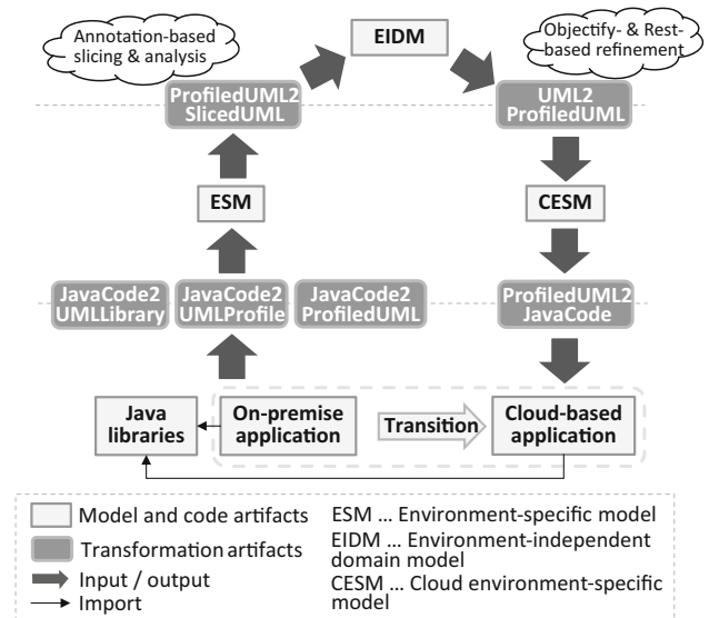
Fig. 16 Modernization roadmap to the cloud
