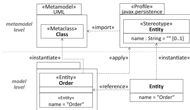
Fig. 4 Application of Entity stereotype
