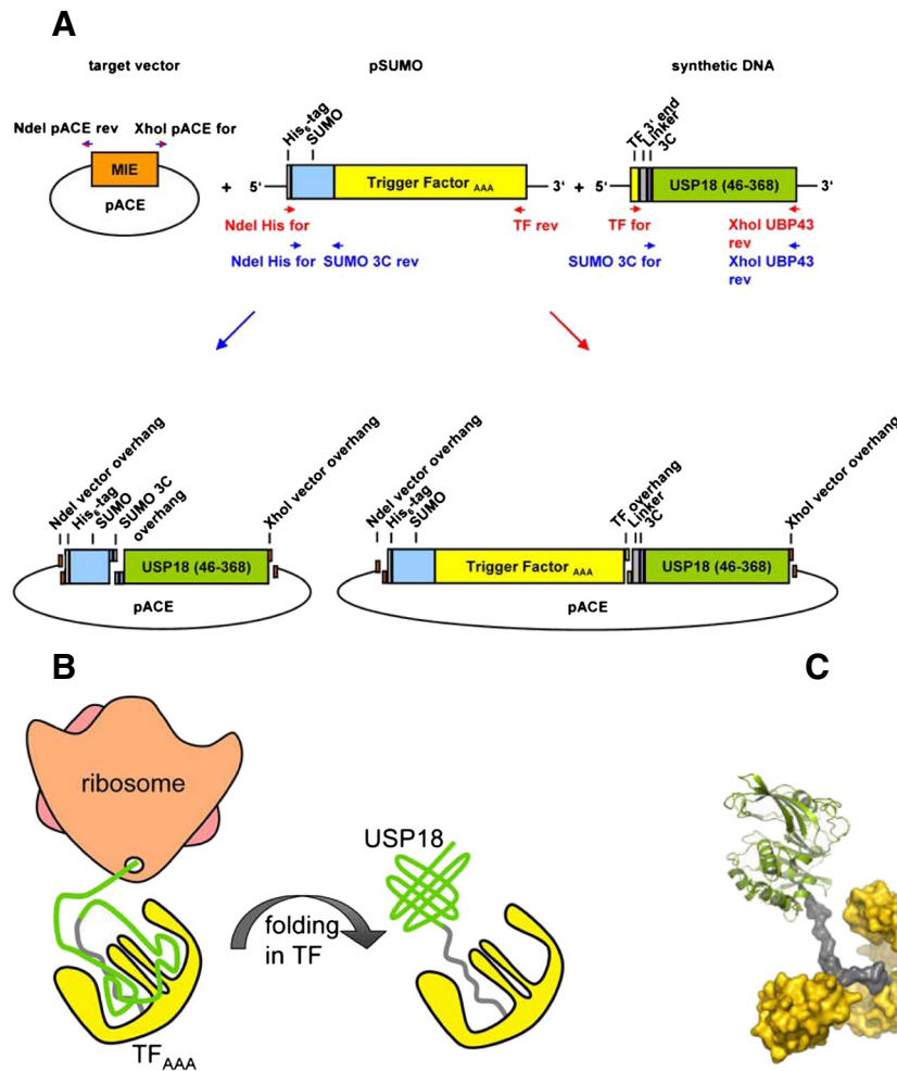
Figure 1 (A) Generation of SUMO-USP18 and SUMO-TF AAA -USP18 expression vectors using sequence and ligation independent cloning (SLIC).
