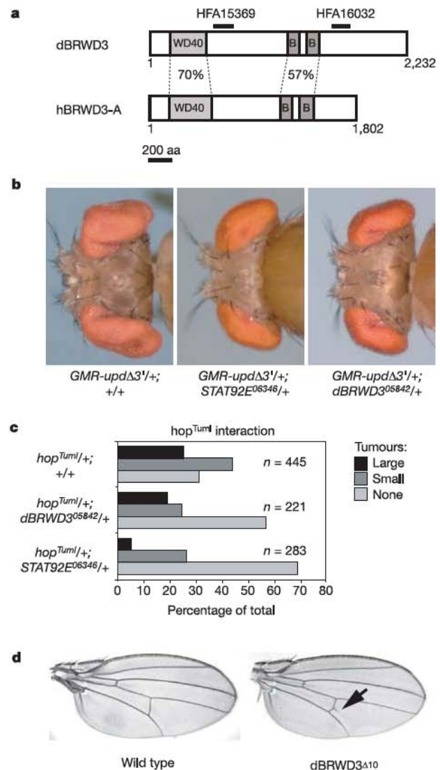
Figure 3 | dBRWD3 functions as a JAK/STAT pathway component. a, Domain structure and sequence similarity of Drosophila and human BRWD3 proteins. Percentages show the similarity in the amino acid sequence, and regions targeted by two independent dsRNAs independently recovered in the screen are shown. b, Adult Drosophila heads heterozygous for the GMR updΔ3' transgene crossed to wild type (left panel), stat92E (middle panel) and dBRWD3 (right panel) mutants. Note the reduction in eye overgrowth after removal of pathway components. c, The size and frequency of hop TumI induced tumour formation is significantly decreased in stat92E and dBRWD3 heterozygous backgrounds. d, Compared to adult wild type wings (left), ectopic wing vein material (arrow) is present in homozygous dBRWD3 Δ10 mutant flies (a putative hypomorphic allele, right), a phenotype reminiscent of the stat92E HJ mutant 12 .
