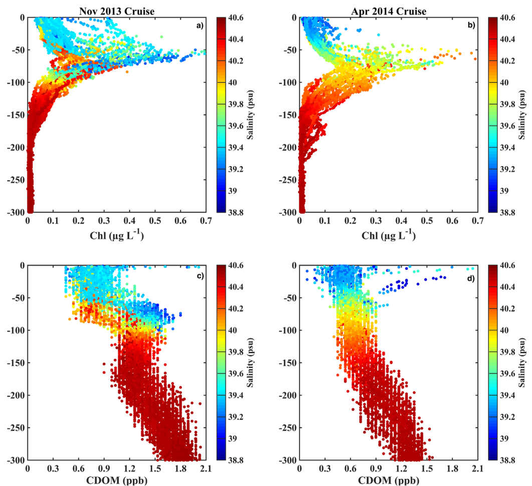
Figure 3. Ship-based vertical profiles of chlorophyll (μg L -1 ), CDOM concentration (ppb), salinity (color-coded) in (a) and (c) November 2013 and (b) and (d) April 2014.
