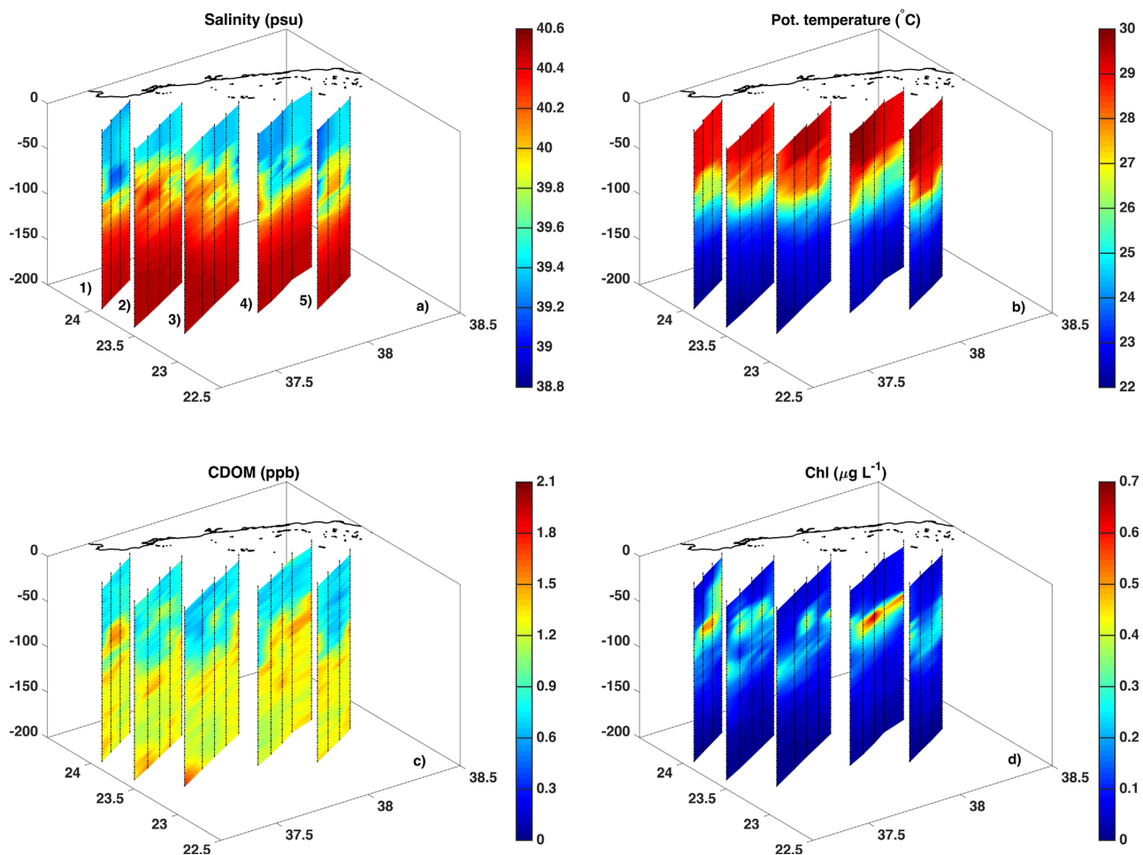
Figure 4. Three-dimensional visualization of (a) salinity, (b) potential temperature (°C), (c) CDOM (ppb), and (d) chlorophyll fluorescence ( \mu\text{g L}^{-1} ) for the five east-west transects of November 2013.
