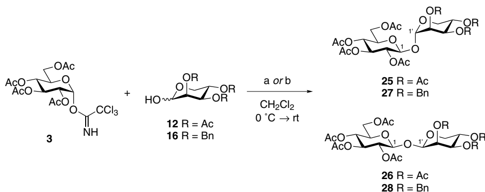
Scheme 5. Synthesis of L-lyxopyranosyl \beta -D-glucopyranosides 25–28 . Reagents: (a) 3 , 12 (1.1 equiv), \text{BF}_3 \cdot \text{OEt}_2 (0.1 equiv) (52%, 25/26 = 1.5:1); (b) 3 (1.4 equiv), 16 , \text{SnCl}_4 (0.03 equiv) (48%, 27/28 = 7:1).
