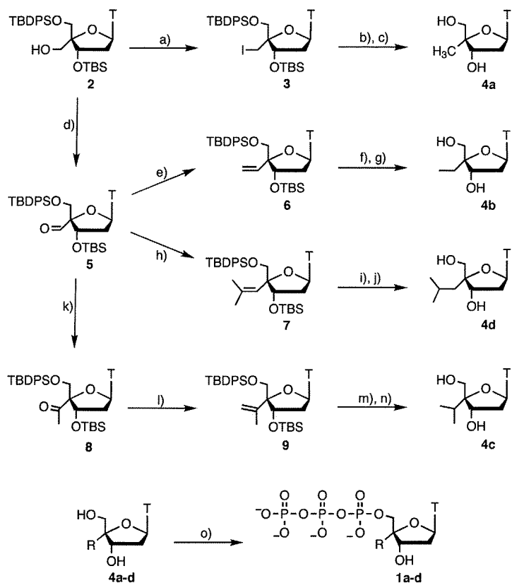
Scheme 2. Syntheses of 1a-d . a) \text{Ph}_3\text{P} , \text{I}_2 , imidazole, \text{C}_6\text{H}_6 , 50^\circ\text{C} , 85%; b) Pd/C, \text{H}_2 , EtOH, EtOAc, \text{NEt}_3 ; c) TBAF, THF, 79% (two steps); d) oxidation; [5] e) \text{CH}_3\text{PPh}_3\text{Br} , n\text{BuLi} , THF, -78 to 25^\circ\text{C} , 99%; f) TBAF, THF; g) Pd/C, \text{H}_2 , \text{CH}_3\text{OH} , 88% (two steps); h) (\text{CH}_3)_2\text{CHPPh}_3\text{I} , n\text{BuLi} , THF, -78 to 25^\circ\text{C} , 83%; i) TBAF, THF; j) Pd/C, \text{H}_2 , \text{CH}_3\text{OH} , 94% (two steps); k) alkylation and oxidation; [5] l) \text{CH}_3\text{PPh}_3\text{Br} , t\text{BuOK} , THF, 25^\circ\text{C} , 91%; m) TBAF, THF; n) Pd/C, \text{H}_2 , \text{CH}_3\text{OH} , 84% (two steps); o) \text{POCl}_3 , 1,8-bis(dimethylamino)naphthalene, (\text{CH}_3\text{O})_3\text{PO} , 0^\circ\text{C} , then (n\text{Bu}_3\text{NH})_2\text{H}_2\text{P}_2\text{O}_7 , n\text{Bu}_3\text{N} , DMF, then 0.1M aqueous (\text{Et}_3\text{NH})\text{HCO}_3 , 23–68%. TBDPS = tert -butyldiphenylsilyl, TBS = tert -butyldimethylsilyl, TBAF = tetrabutylammonium fluoride, THF = tetrahydrofuran, DMF = N,N -dimethylformamide.
