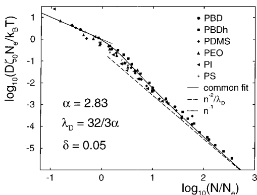
Figure 4. Self-diffusion constants for polymer melts versus reduced molecular weight. A common fit for the data of different polymers with the indicated parameters is shown as a solid line. The asymptotes, Rouse and reptation-like, are shown with prefactors corresponding to the fit.
