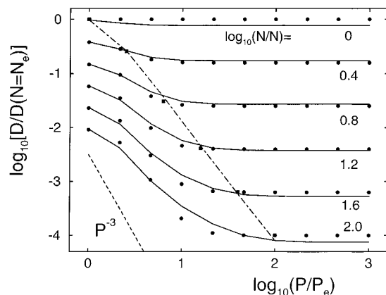
Figure 5. Tracer diffusion coefficients versus matrix molecular weight, p = P/P_e , for different tracer molecular weights, n = N/N_e , as specified in the figure. The model of Graessley, 12 eq 1, which has been fitted to polystyrene (PS) melts by Green and Kramer, 66 is shown by circles for n \neq p and by squares for n = p . The PMC fit is shown by the solid curves; parameters are \alpha = 3 (a priori fixed), \delta = 0.07 , and \lambda_D = 1.58 . The corresponding self-diffusion coefficients are indicated by a chain curve.
