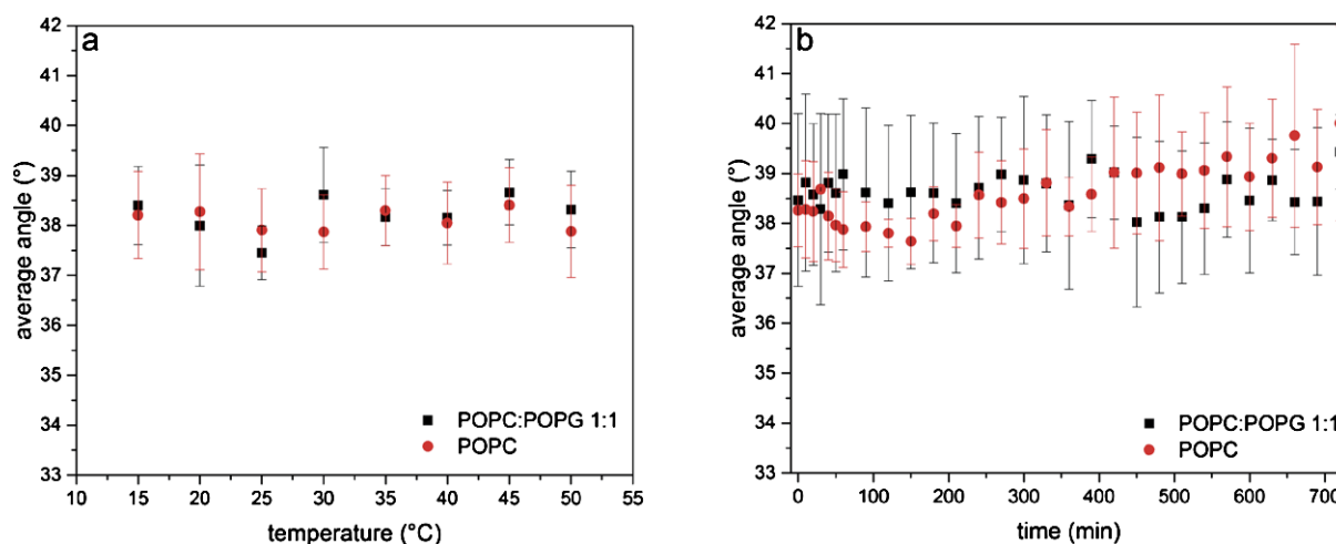
Fig. 2. Stability of SSLBs at different temperatures and over time. The orientation of the lipid alkyl chains with respect to the surface normal of a mixture of POPC and POPG (black squares) and of pure POPC (red circles) is shown (a) for different temperatures and (b) over 12 h at 25°C.
