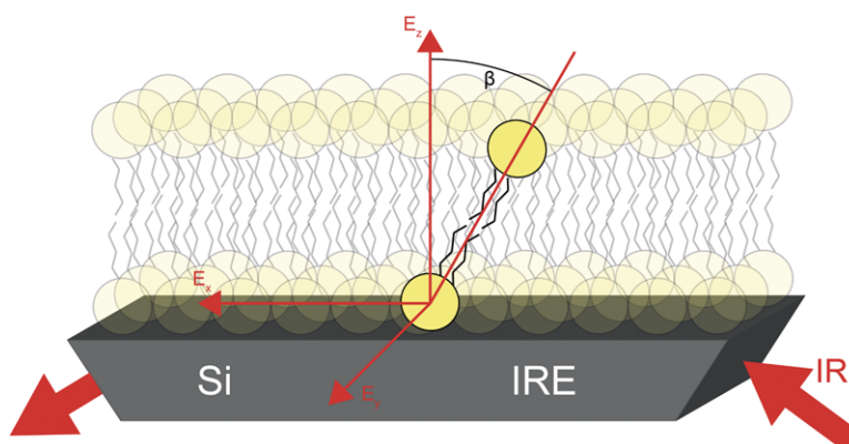
Fig. 1. Schematic representation of the lipid orientation within a SSLB. The determined average angle \beta is illustrated at a highlighted lipid molecule. E_{xyz} are the components of the electric field vector of the evanescent IR wave. \beta represents an average value for all lipids present in the sample.
