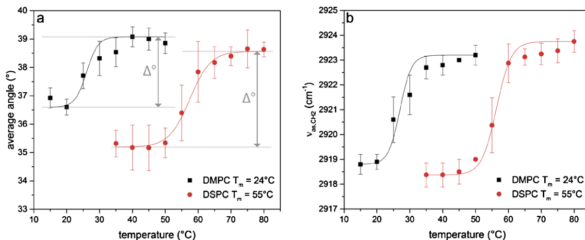
Fig. 3. Changes upon lipid phase transition of DMPC and DSPC. Investigation of (a) the orientation of the lipid alkyl chain and (b) the frequency position of the band corresponding to the asymmetric stretching vibration of the \text{CH}_2 -groups ( \nu_{\text{as,CH}_2} ) in the lipid alkyl chain for DMPC (black squares) and DSPC (red circles) respectively. The data were fitted to determine the phase transition temperature and the difference in the average angle for both phases ( \Delta^\circ ).
