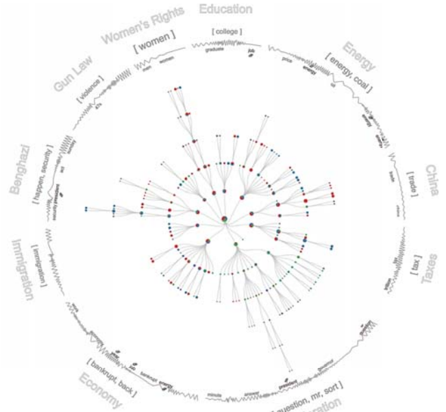
Fig. 5: IHTM result (with backbone; supervised SpecEx optimizations; no direct tree manipulations) for the second presidential debate between Romney and Obama in 2012 [17] in our topic-tree visualization.
