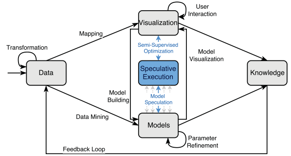
Fig. 6: Extension of VA-Pipeline by Keim et al. [38] to SpexEx-VA , with speculative execution as semi-supervised optimization technique.
