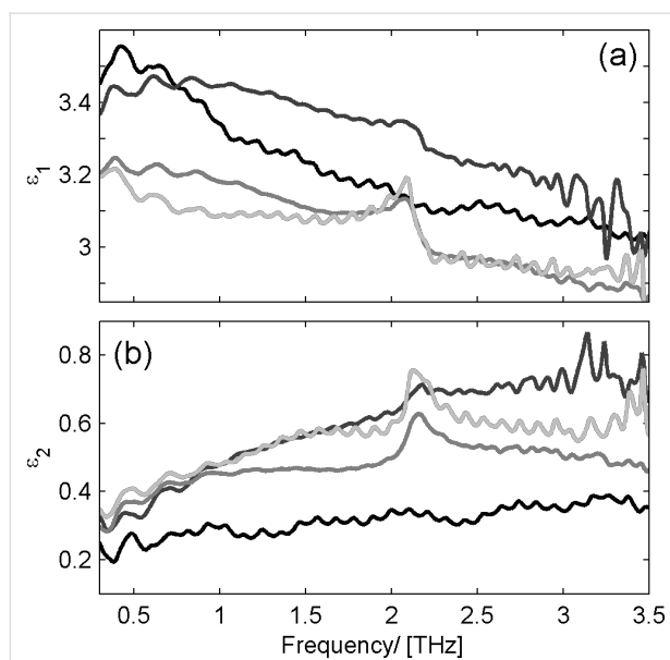
Figure 1: Figure 8 in the original article: Measured dielectric function of \text{ZnO}_{1-x}\text{Cl}_x (a) real part; (b) imaginary part with x = 0.0\% (black lines), 1.4\% (dark gray lines), 1.8\% (gray lines) and 2.5\% (light gray lines); An infrared-active phonon at about 2 THz is scaling in intensity with increasing Cl concentration.
