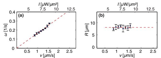
FIG. 2 (color online). (a) Angular velocity \omega and (b) radius R of the circular motion of an L+ swimmer plotted as functions of the linear velocity v = |\mathbf{v}| and the illumination intensity I \sim v . The dashed lines correspond to a linear fit with nonzero and zero slope, respectively.
