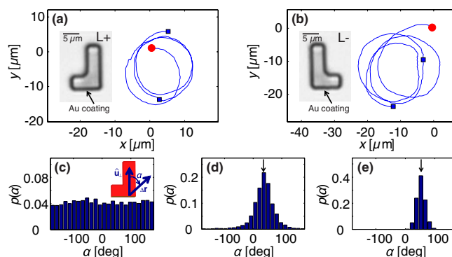
FIG. 1 (color online). (a),(b) Trajectories of an (a) L + and (b) L − swimmer for an illumination intensity of 7.5 \mu\text{W}/\mu\text{m}^2 . (Red) bullets and (blue) square symbols correspond to initial particle positions and those after 1 min each, respectively. The insets show microscope images of two different swimmers with the Au coating (not visible in the bright-field image) indicated by an arrow. (c),(d),(e) Probability distributions p(\alpha) of the angle \alpha [see inset in (c)] between the normal vector \hat{\mathbf{u}}_{\perp} of the metal coating and the displacement vector \Delta\mathbf{r} of an L + particle in time intervals of 12 s each for illumination intensities (c) I = 0 \mu\text{W}/\mu\text{m}^2 , (d) 5 \mu\text{W}/\mu\text{m}^2 and (e) 7.5 \mu\text{W}/\mu\text{m}^2 .
