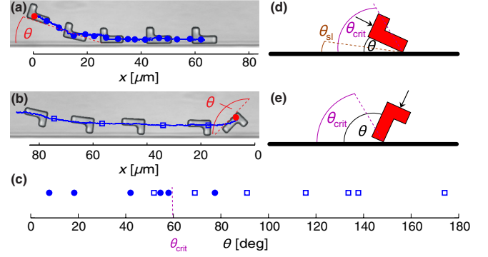
FIG. 4 (color online). (a),(b) Trajectories of an L+ swimmer approaching a straight wall at different angles (symbols correspond to positions after 1 min each). (c) Experimentally determined particle motion for different contact angles \theta . Bullets and open squares correspond to particle sliding and reflection. (d), (e) Visualization of the predicted types of motion for an L+ swimmer with arrows indicating the direction of the propulsion force: (d) stable sliding and (e) reflection. The angles are defined in the text.
