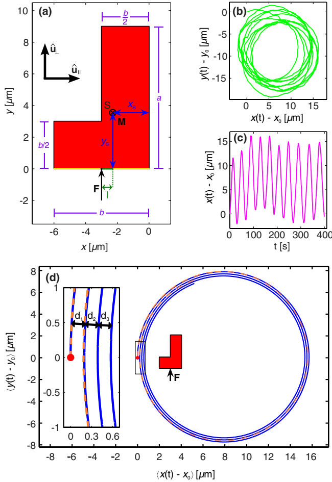
FIG. 3 (color online). (a) Geometrical sketch of an ideal L +swimmer as considered in our model. The dimensions are a = 9 \mu\text{m} , b = 6 \mu\text{m} , x_S = 2.29 \mu\text{m} , and y_S = 3.55 \mu\text{m} (for homogeneous mass density and an additional 20 nm thick Au layer). The internal force \mathbf{F} induces a torque \mathbf{M} on the center-of-mass S depending on the lever arm l . (b),(c) Visualization of the experimental trajectory (for an illumination intensity of I = 7.5 \mu\text{W}/\mu\text{m}^2 ) that is used for the quantitative analysis of the fluctuation-averaged trajectory in (d). The dashed curve in (d) is the experimental one, and the solid curve shows the theoretical prediction with the starting point indicated by a red bullet. Inset: closeup of the framed area in the plot.
