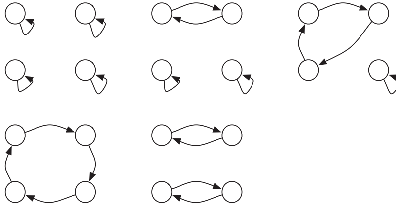
Fig. 3. Cycle Types of S_4 .
