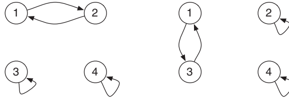
Fig. 1. Functions f (left) and g (right).
