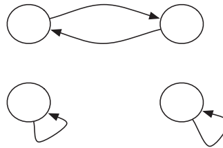
Fig. 2. Function on Cardinal Four Structure.
