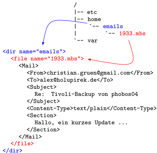
Figure 3: From file hierarchy to relational storage. Translators include file content to allow content and structure based queries as well as the deep access functionality while navigating along the file hierarchy.
