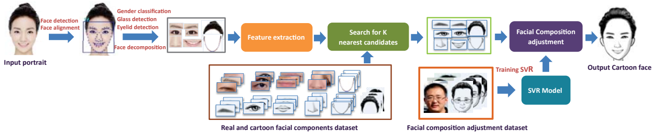
Figure 2: The overall pipeline of our framework.
