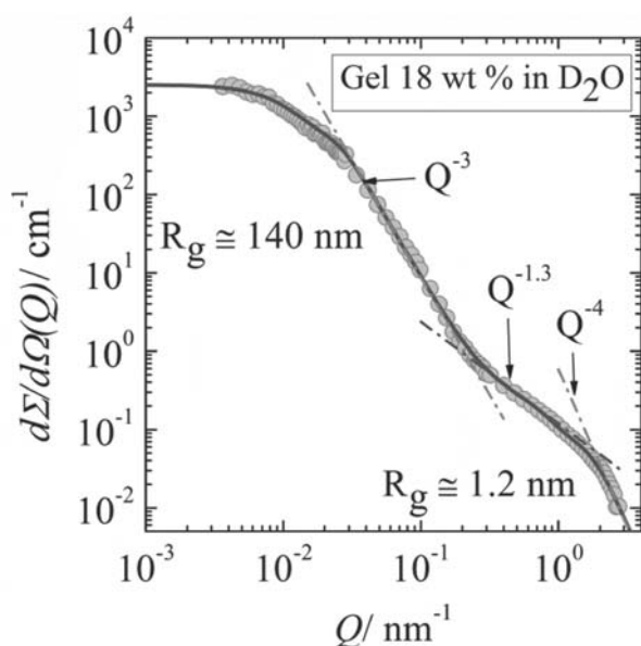
Figure 1. SANS macroscopic cross-section d\Sigma/d\Omega versus scattering vector Q for 18 wt% gelatin in D_2O ( T = 20\text{ }^\circ\text{C} ). At low Q ( < 0.02\text{ nm}^{-1} ) USANS data are also presented after rescaling. The solid line represents a fit of the two levels Beaucage equation.
