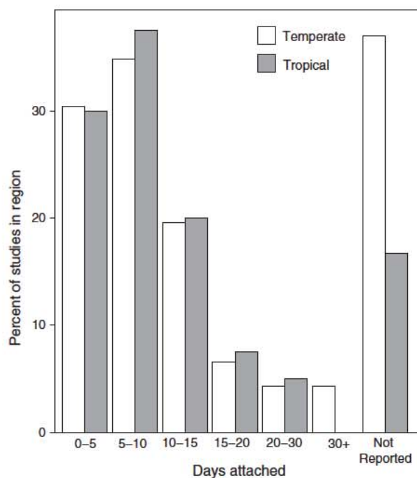
Fig. 1. Duration of transmitter attachment in temperate and tropical studies as a percentage of the total studies in each region, excluding those studies where data were not available. Studies where data were not reported are presented as a percentage of the total number of studies returned in the search.
