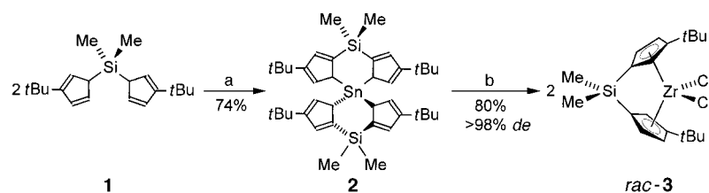
Scheme 1. Stereoselective formation of rac - 3 via the bicyclic tin compound 2 : a) Sn(NMe_2)_4 , Et_2O , room temperature; b) ZrCl_4 , toluene, room temperature.
