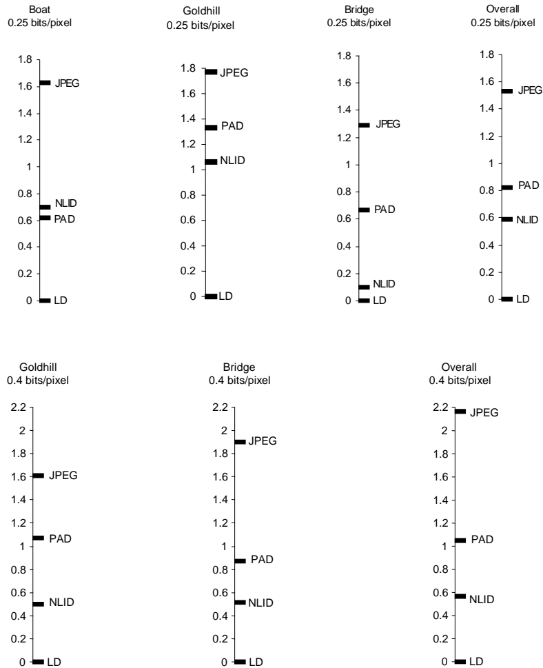
Figure 2 Scaling results. The scales show the expected values of a model observers quality assessment with respect to a chosen reference point, e.g., the position of LD. Positive difference on the scale means “better in expectance”. The unit is the uncertainty of the decision. Large differences mean a better discrimination.
