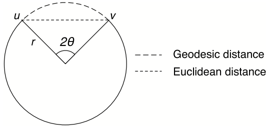
Fig. 1. Euclidean and geodesic distances on a circle.
