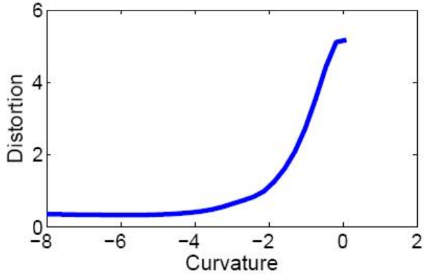
Fig. 2. The distortion of embedding the internet in dimension two as a function of the curvature of the embedding space [19].
