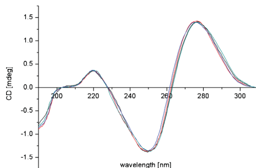
Fig. 4 CD-spectra of unmodified DNA (—) and adamantane modified DNA (—), diamantane modified DNA (—) and triamantane modified DNA (—). The CD spectra show the characteristic profile of a B-DNA with a positive maximum at about 275 nm and a minimum at about 250 nm. Compared to the unmodified oligonucleotides the curve of the modified ones do not show significant differences.
